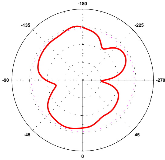
E Plane
