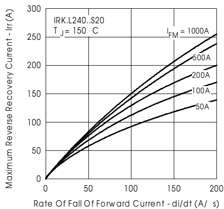
Fig. 18-ReverseRecoveryCurrentCharacteristics
