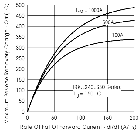
Fig. 19-ReverseRecoveryChargeCharacteristics
