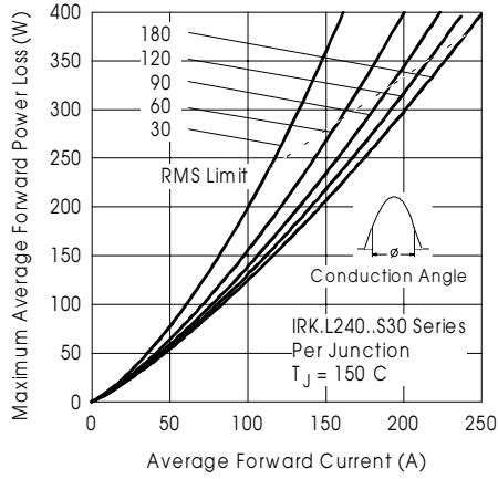
Fig.9-ForwardPowerLossCharacteristics
