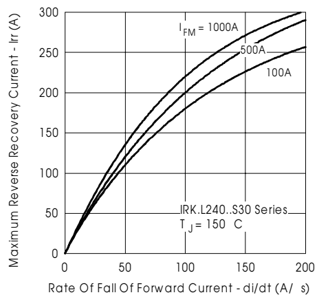
Fig. 20-ReverseRecoveryCurrentCharacteristics
