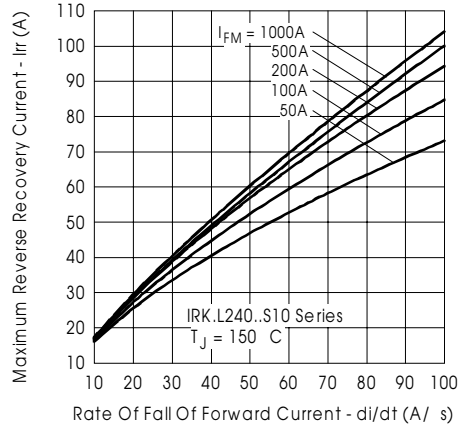
Fig. 16-ReverseRecoveryCurrentCharacteristics
