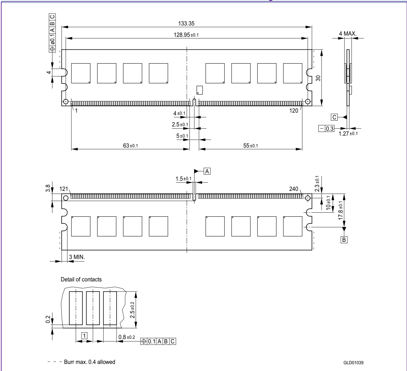
FIGURE 8 Package Outline Raw Card E L-DIM-240-9
