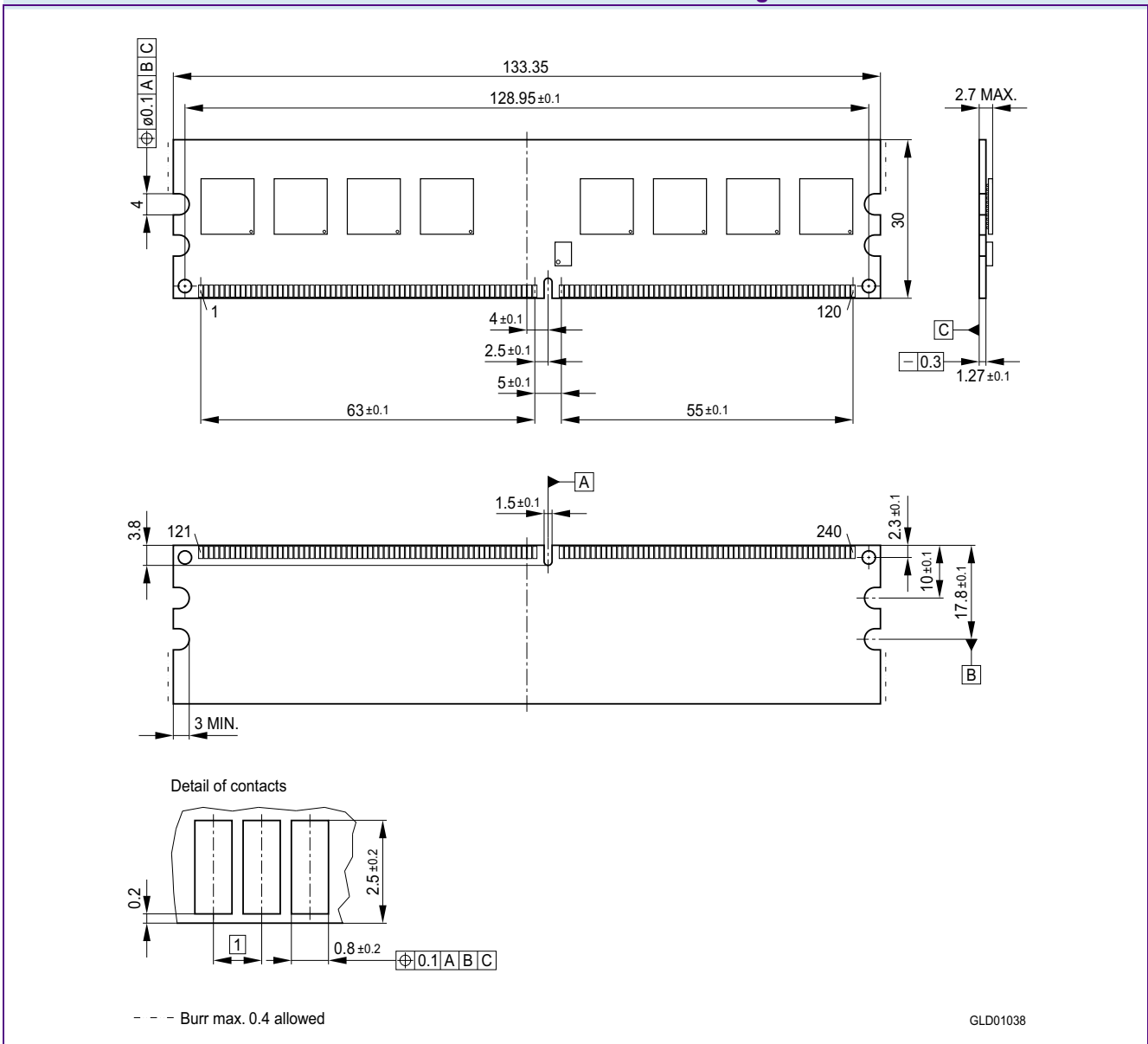
FIGURE 7 Package Outline Raw Card D L-DIM-240-8
