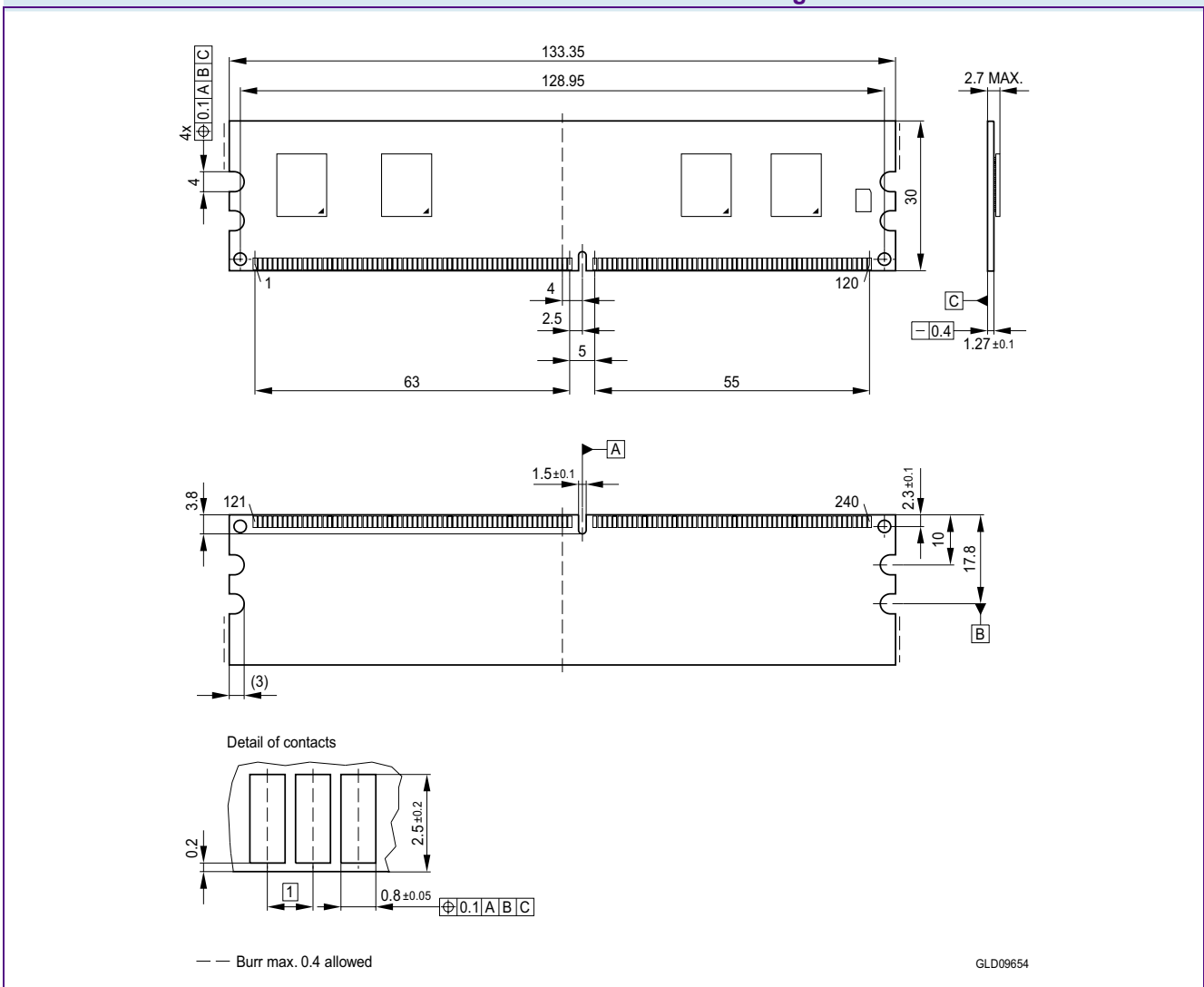
FIGURE 6 Package Outline Raw Card C L-DIM-240-3
