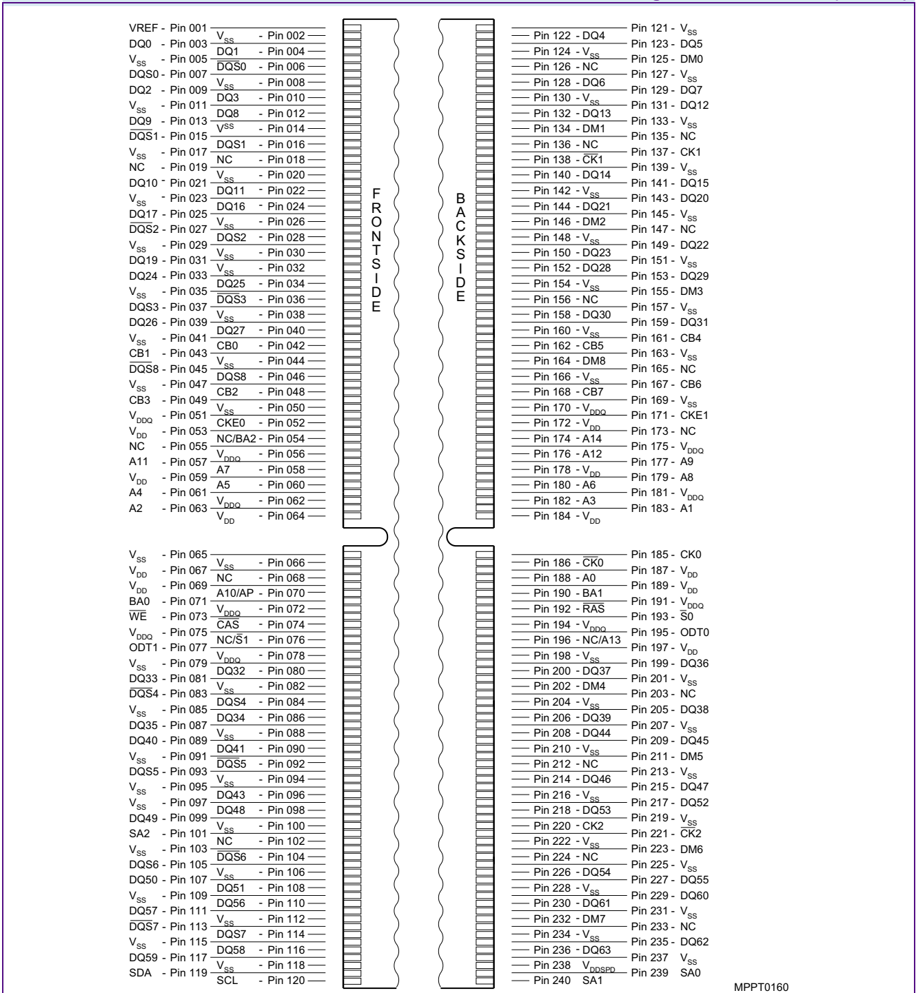
FIGURE 2 Pin Configuration UDIMM x72 (240 Pin)
