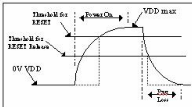
Figure 18: Power-on-Reset Characteristics
