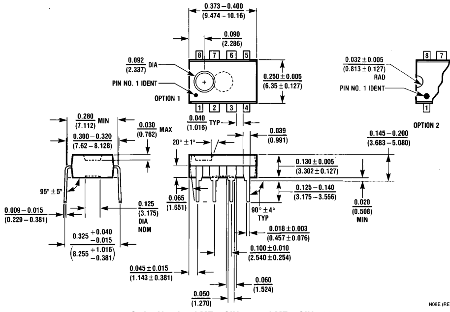
Order Number LMF40CIN-50, or LMF40CIN-100 NS Package Number N08E
