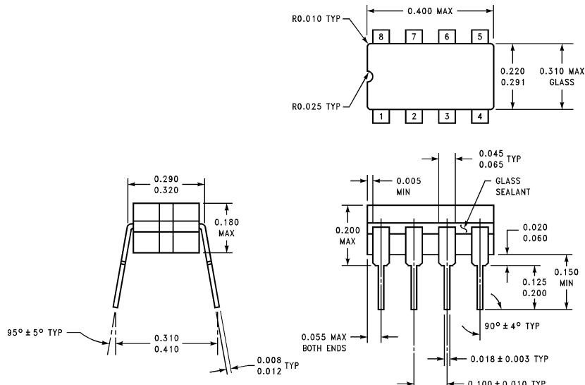
Order Number LMF40CMJ-50 or LMF40CMJ-100 NS Package Number J08A
