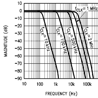
FIGURE 5c. LMF40-100 Amplitude Response with \pm 2.5V Supplies
