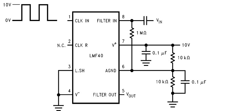
FIGURE 3. Single Supply Operation. AGND Resistor Biased to V^+ / 2
