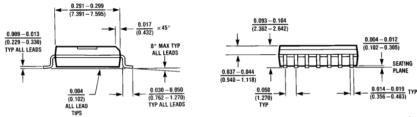
Order Number LMF40CIWM-50 or LMF40CIWM-100 NS Package Number M14B
