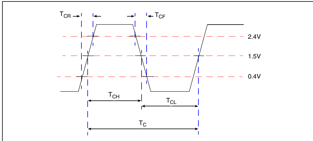
Figure 7. MCLK Waveform
