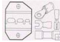
Die for Barrel Type Connectors 22-10 AWG Insulated
