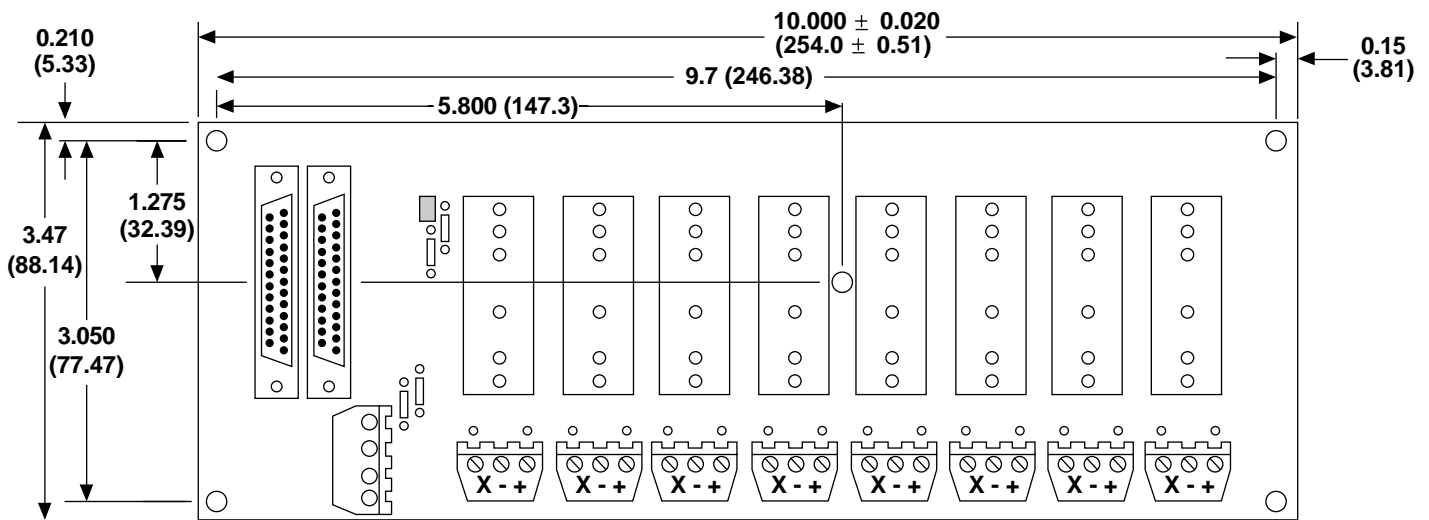
Model 7BP08-1 Backplane.
