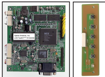
B TFT Controller Board with On-Screen Display (OSD) Board (VNS-AV-104VGATTL-00)
