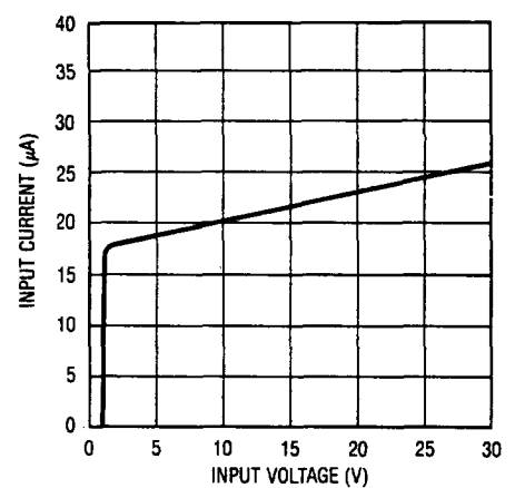
Input Current
