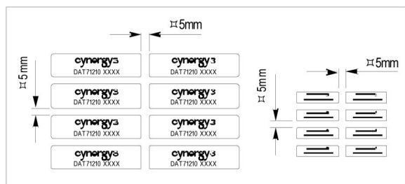
Figure 4 : Recommended Mounting for "S" and "D" Series High Voltage Reed Relays
