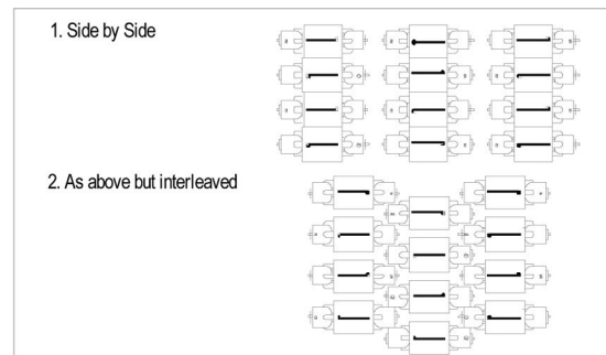
Figure 3 : Mounting Configurations to Minimise Magnetic Interference (Note Orientation)
