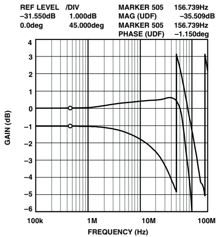
TPC 4. Frequency and Phase Response vs. Gain (Gain = +30 dB, P_{IN} = -30 dBm, Pin 5 Connected to Pin 7)
