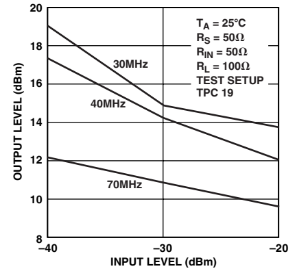
TPC 24. Third Order Intercept, -10 dB/+30 dB Mode, Gain = +30 dB
