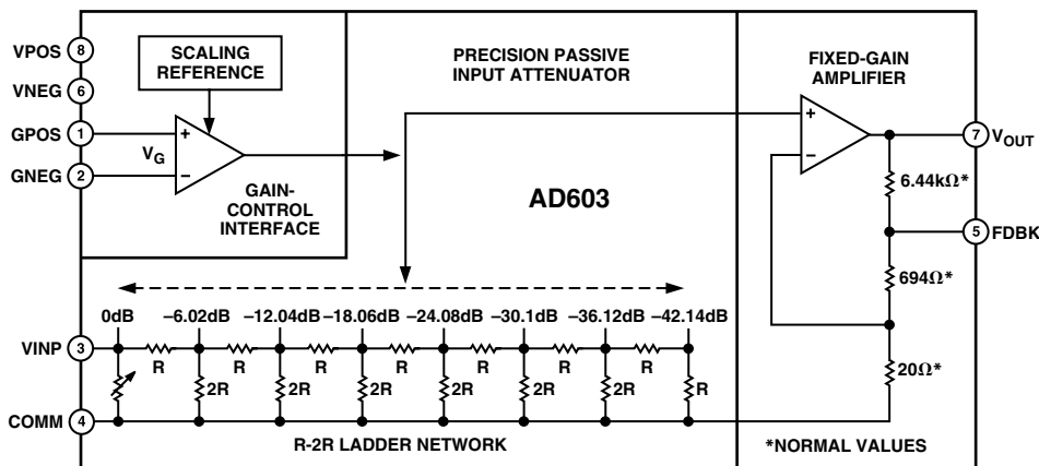
Figure 1. Simplified Block Diagram
