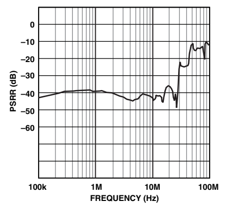
TPC 18. PSRR vs. Frequency (Worst Case Is Negative Supply PSRR, Shown Here)
