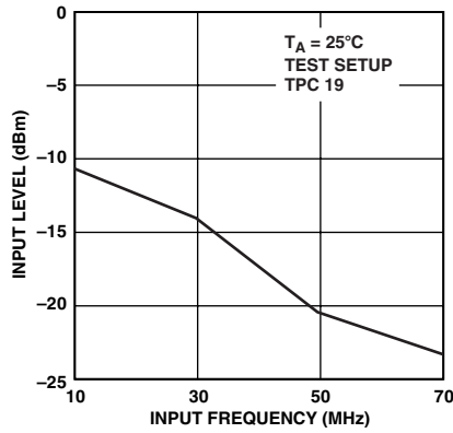
TPC 22. 1 dB Compression Point, -10 dB/+30 dB Mode, Gain = +30 dB
