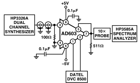
TPC 6. Third Order Intermodulation Distortion Test Setup
