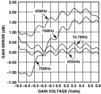
TPC 1. Gain Error vs. Gain Control Voltage at 455 kHz, 10.7 MHz, 45 MHz, 70 MHz
