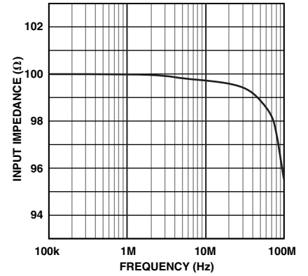
TPC 12. Input Impedance vs. Frequency (Gain = +30 dB)
