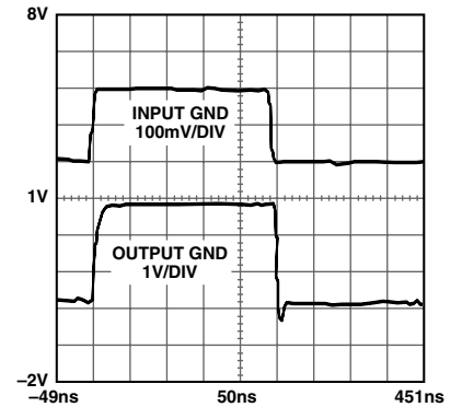
TPC 15. Output Stage Overload Recovery Time, Pin 5 Connected to Pin 7 (Input Is 500 ns Period, 50% Duty-Cycle Square Wave, Output Is Captured Using Tektronix 11402 Digitizing Oscilloscope)
