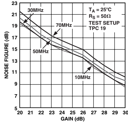
TPC 20. Noise Figure in -10 dB/+30 dB Mode
