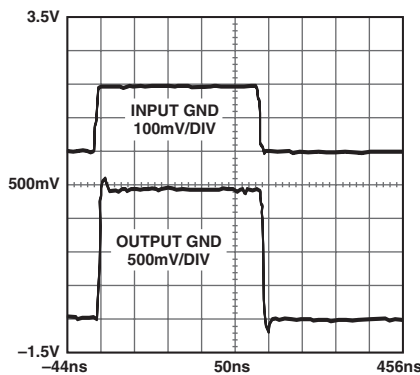
TPC 17. Transient Response, G = +20 dB, Pin 5 Connected to Pin 7 (Input Is 500 ns Period, 50% Duty-Cycle Square Wave, Output Is Captured Using Tektronix 11402 Digitizing Oscilloscope)
