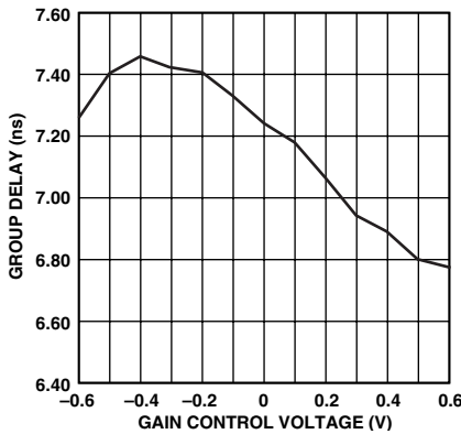
TPC 5. Group Delay vs. Gain Control Voltage
