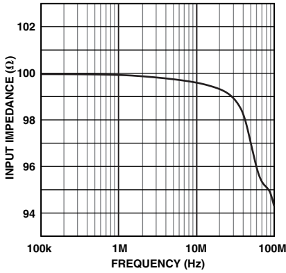
TPC 10. Input Impedance vs. Frequency (Gain = -10 dB)
