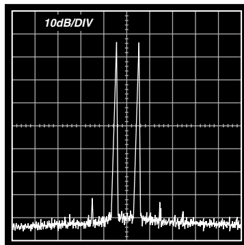
TPC 8. Third Order Intermodulation Distortion at 10.7 MHz (10× Probe Used to HP3585A Spectrum Analyzer, Gain = 0 dB, P_{IN} = 0 dBm, Pin 5 Connected to Pin 7)
