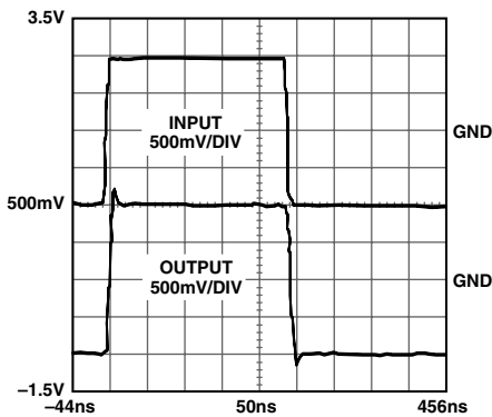
TPC 16. Transient Response, G = 0 dB, Pin 5 Connected to Pin 7 (Input Is 500 ns Period, 50% Duty-Cycle Square Wave, Output Is Captured Using Tektronix 11402 Digitizing Oscilloscope)
