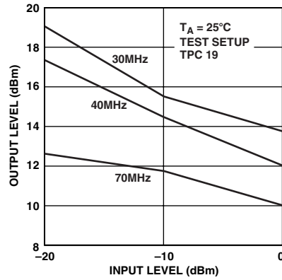
TPC 23. Third Order Intercept -10 dB/+30 dB Mode, Gain = +10 dB
