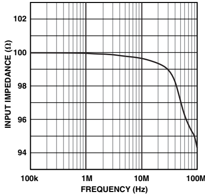
TPC 11. Input Impedance vs. Frequency (Gain = +10 dB)
