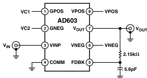
b. 0 dB to 40 dB; 30 MHz Bandwidth
