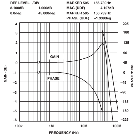
TPC 2. Frequency and Phase Response vs. Gain (Gain = -10 dB, P_{IN} = -30 dBm, Pin 5 Connected to Pin 7)
