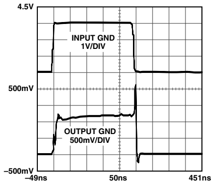
TPC 14. Input Stage Overload Recovery Time, Pin 5 Connected to Pin 7 (Input Is 500 ns Period, 50% Duty-Cycle Square Wave, Output Is Captured Using Tektronix 11402 Digitizing Oscilloscope)
