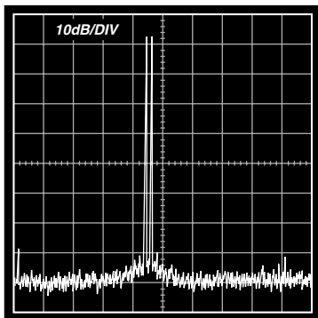
TPC 7. Third Order Intermodulation Distortion at 455 kHz (10× Probe Used to HP3585A Spectrum Analyzer, Gain = 0 dB, P_{IN} = 0 dBm, Pin 5 Connected to Pin 7)
