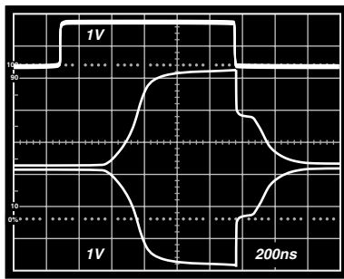
TPC 13. Gain-Control Channel Response Time
