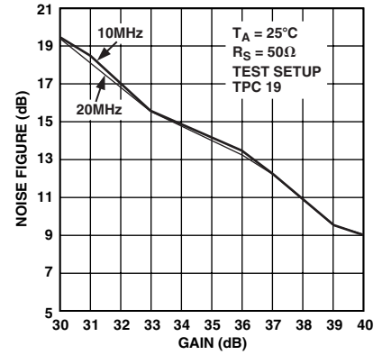
TPC 21. Noise Figure in 0 dB/40 dB Mode
