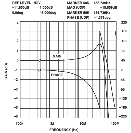
TPC 3. Frequency and Phase Response vs. Gain (Gain = +10 dB, P_{IN} = -30 dBm, Pin 5 Connected to Pin 7)
