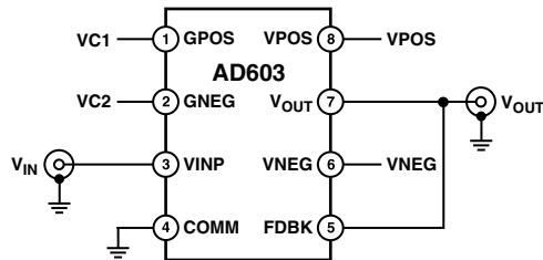
a. -10 dB to +30 dB; 90 MHz Bandwidth
