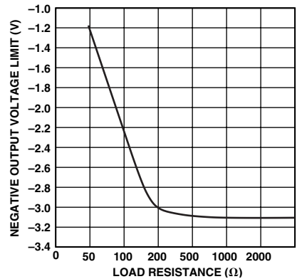
TPC 9. Typical Output Voltage Swing vs. Load Resistance (Negative Output Swing Limits First)
