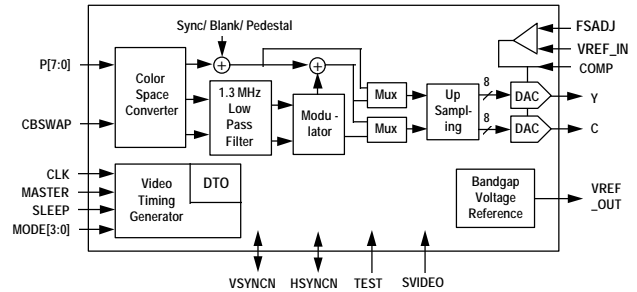
Figure-1 W9952QP Functional Block
