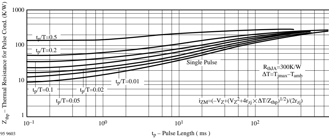
Figure 11. Thermal Response
