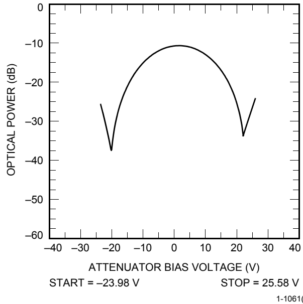
Figure 6. Optical Power vs. Attenuator Bias Voltage
