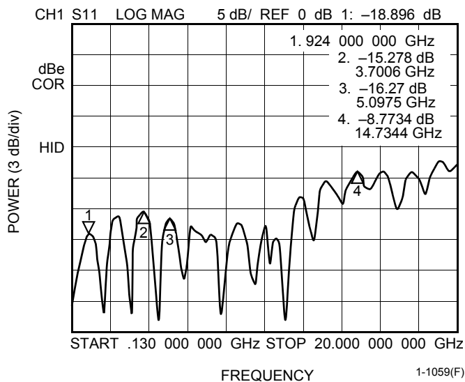
Figure 4. S11, 0.130 GHz—20 GHz
