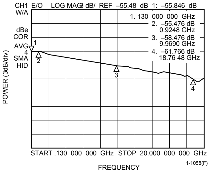
Figure 3. Magnitude of Electro-Optic Response, 0.130 GHz—20 GHz.
