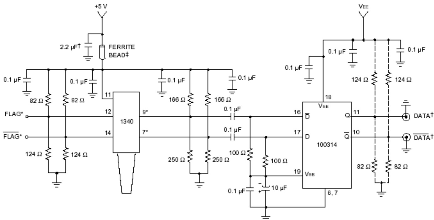
Figure 4. Interfacing to the 622 Mb/s and 1.25 Gb/s 1340 Receivers
