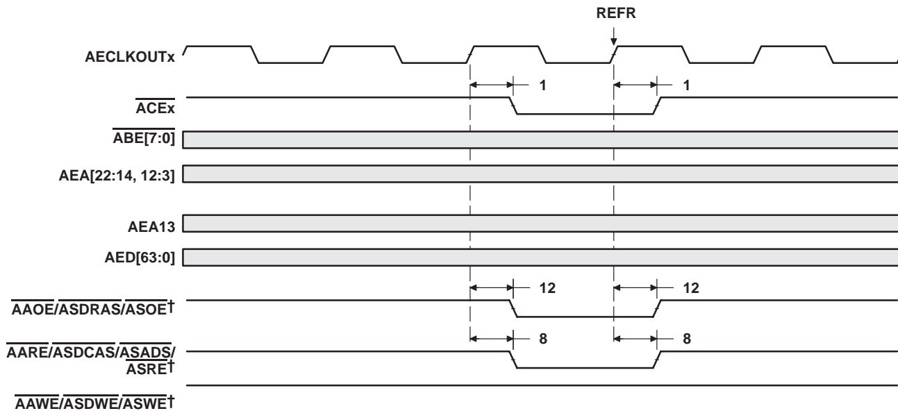
Figure 5–17. SDRAM REFR Command for EMIFA
