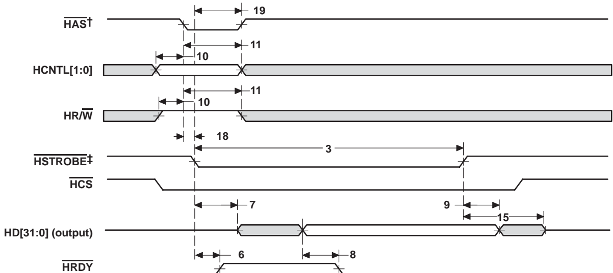
Figure 5–33. HPI32 Read Timing ( \overline{\text{HAS}} Used)
