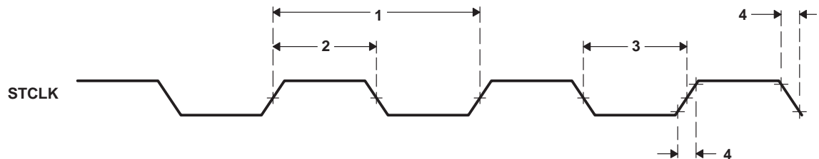
Figure 5–48. STCLK Timing
