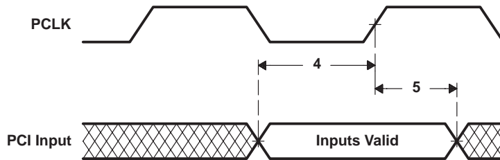
Figure 5–38. PCI Input Timing (33-/66-MHz)
