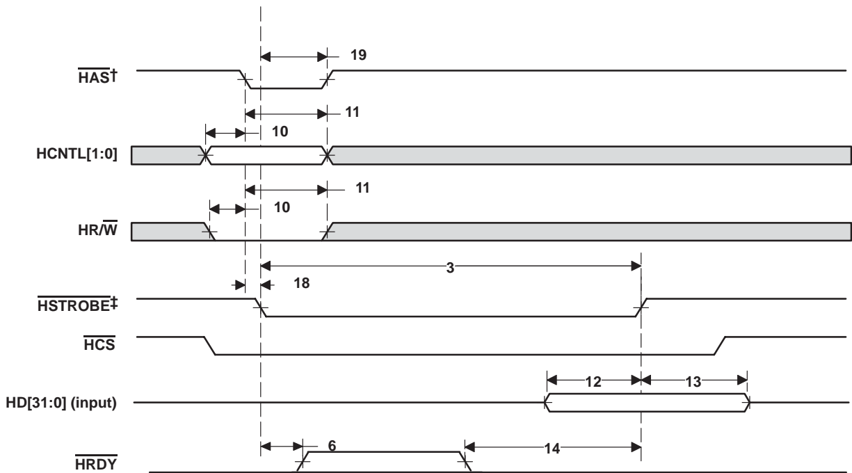
Figure 5–35. HPI32 Write Timing ( \overline{\text{HAS}} Used)
