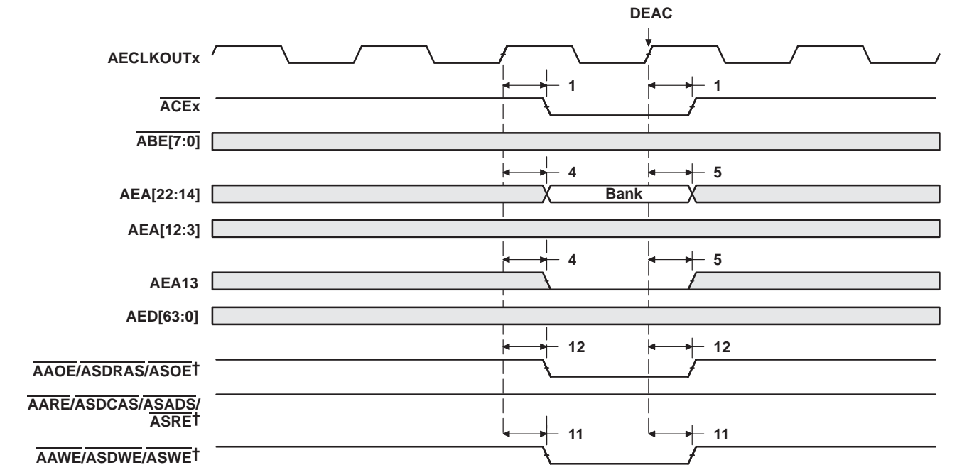
Figure 5–16. SDRAM DEAC Command for EMIFA
