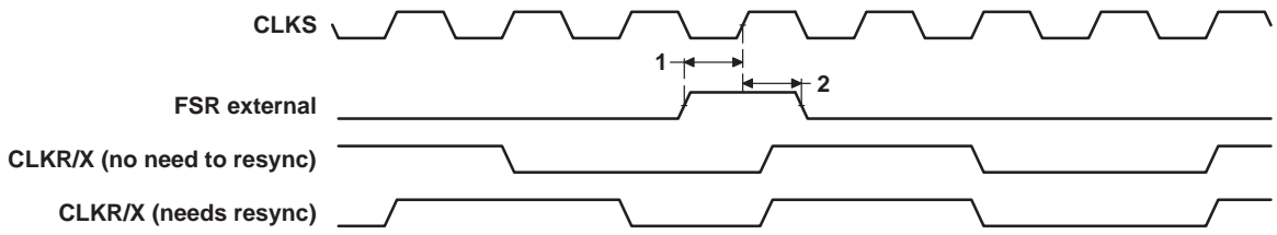
Figure 5-42. FSR Timing When GSYNC = 1
