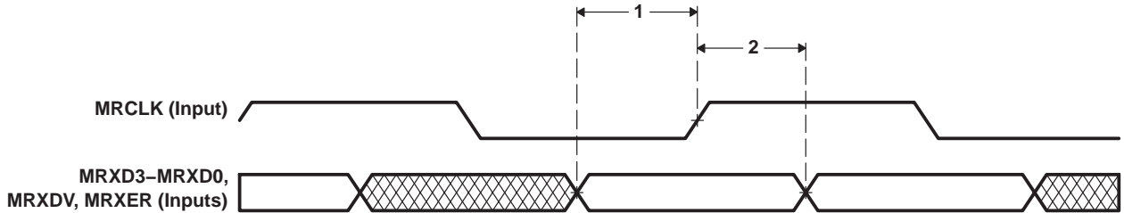
Figure 5–55. EMAC Receive Interface Timing
