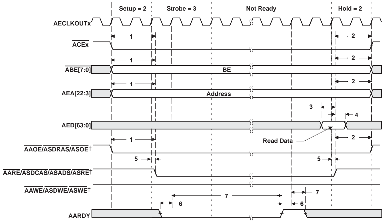
Figure 5–7. Asynchronous Memory Read Timing for EMIFA
