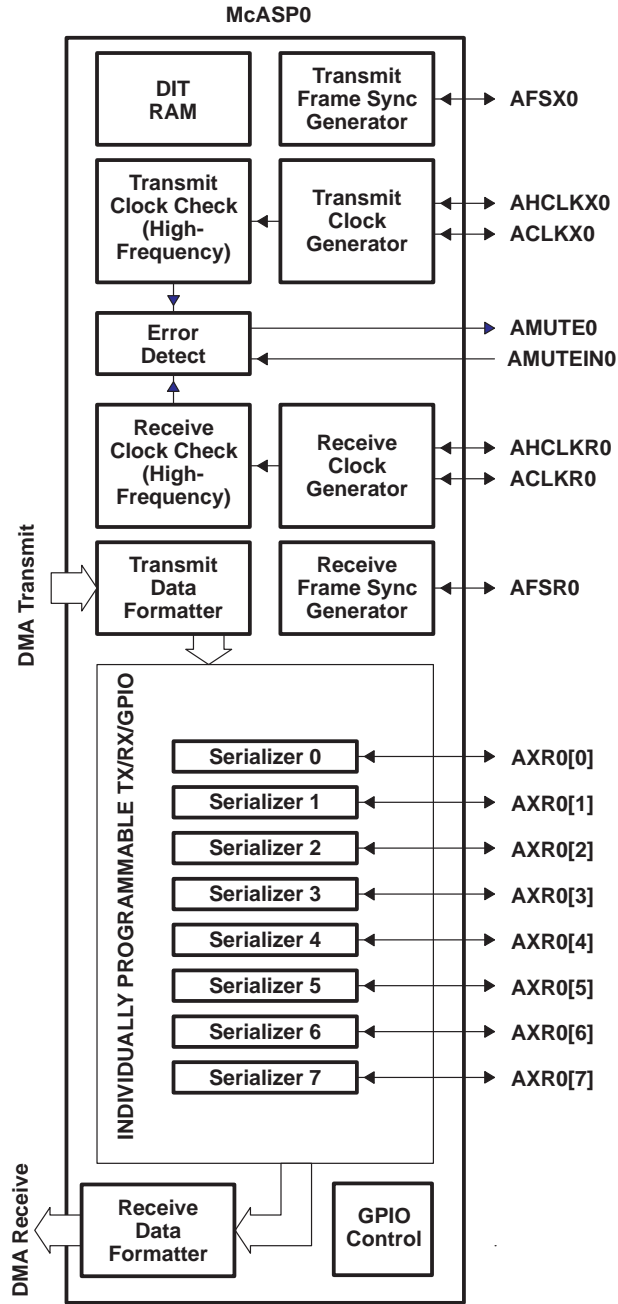
Figure 2–12. McASP0 Configuration
