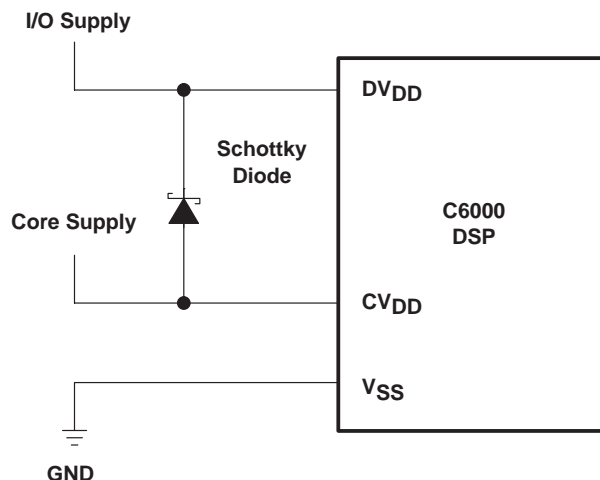
Figure 2–18. Schottky Diode Diagram
