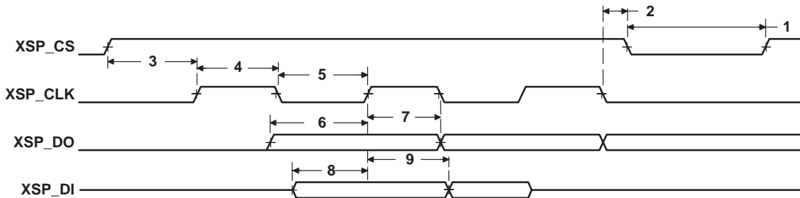
Figure 5–40. PCI Serial EEPROM Interface Timing
