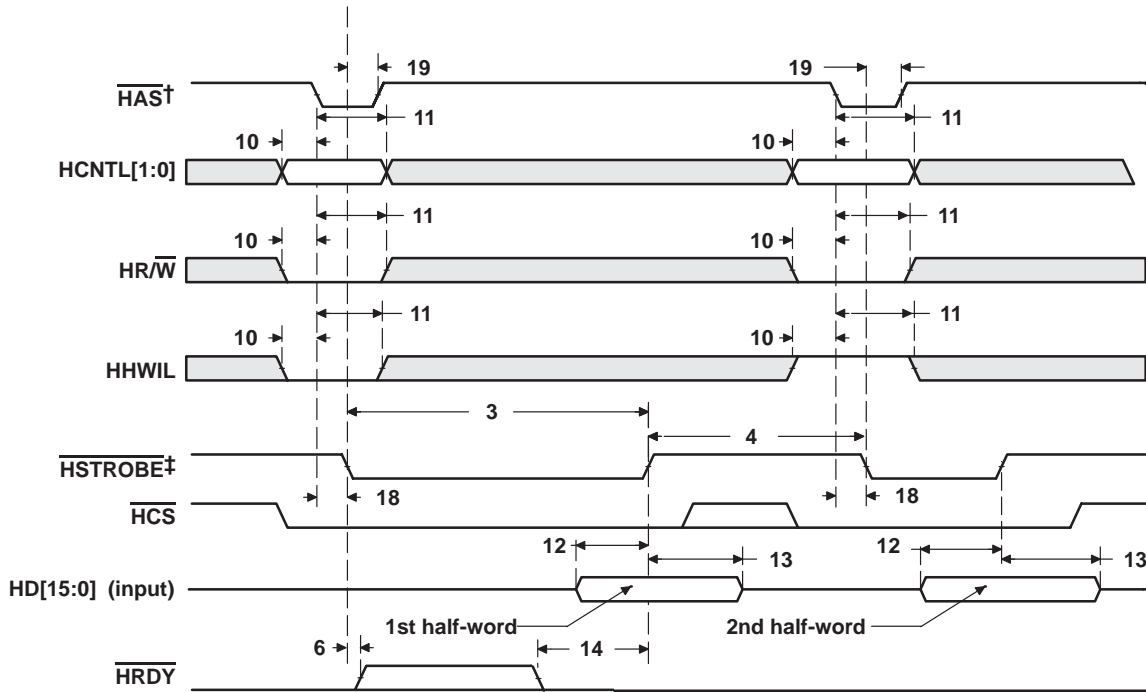
Figure 5–31. HPI16 Write Timing ( \overline{\text{HAS}} Used)
