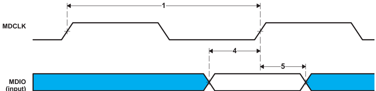
Figure 5-57. MDIO Input Timing
