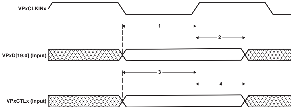
Figure 5–49. Video Port Capture Data and Control Input Timing
