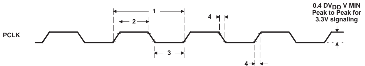
Figure 5–36. PCLK Timing
