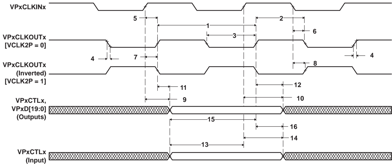
Figure 5–51. Video Port Display Data Output Timing and Control Input/Output Timing With Respect to VPxCLKINx and VPxCLKOUTx
