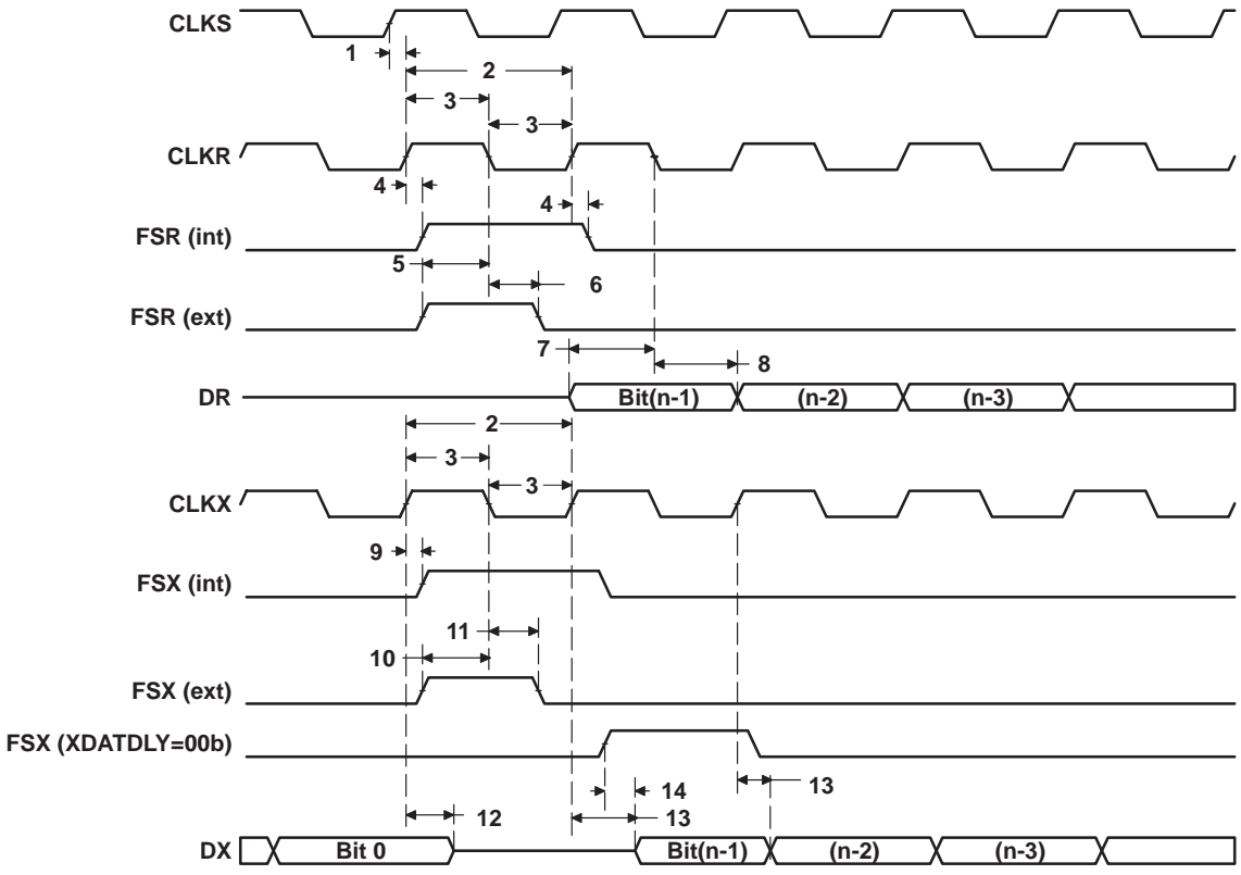
Figure 5-41. McBSP Timing
