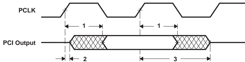
Figure 5–39. PCI Output Timing (33-/66-MHz)
