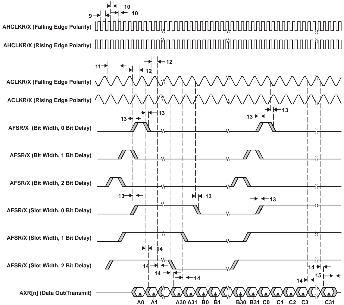
Figure 5–25. McASP Output Timings
