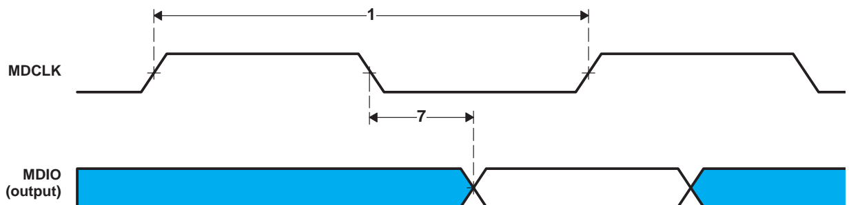
Figure 5-58. MDIO Output Timing
