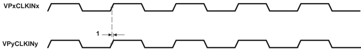
Figure 5–52. Video Port Dual-Display Sync Timing
