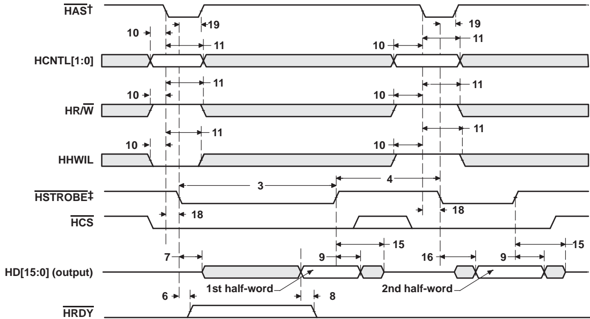
Figure 5–29. HPI16 Read Timing ( \overline{\text{HAS}} Used)
