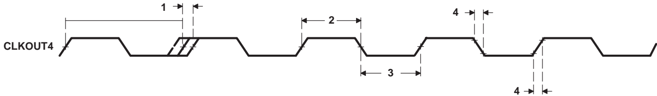
Figure 5–2. CLKOUT4 Timing
