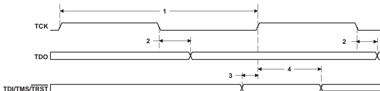
Figure 5–61. JTAG Test-Port Timing
