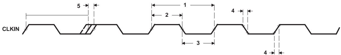
Figure 5–1. CLKIN Timing
