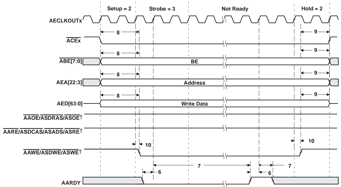
Figure 5–8. Asynchronous Memory Write Timing for EMIFA
