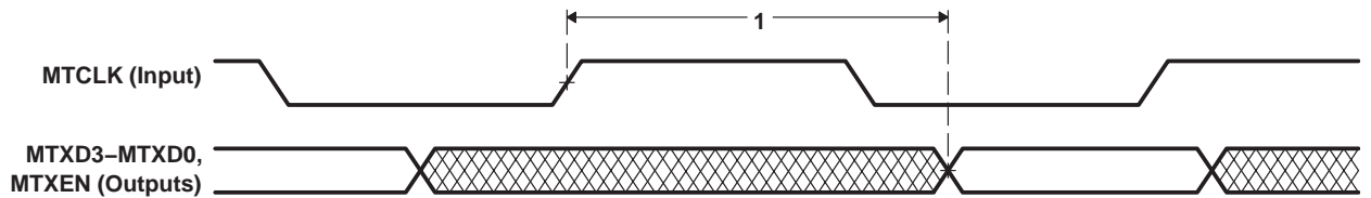
Figure 5–56. EMAC Transmit Interface Timing
