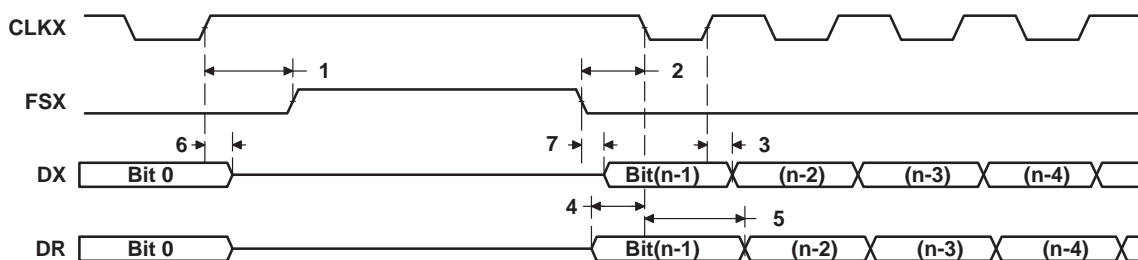
Figure 5–46. McBSP Timing as SPI Master or Slave: CLKSTP = 11b, CLKXP = 1
