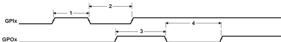
Figure 5–60. GPIO Port Timing
