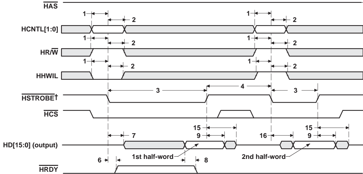
Figure 5–28. HPI16 Read Timing ( \overline{\text{HAS}} Not Used, Tied High)
