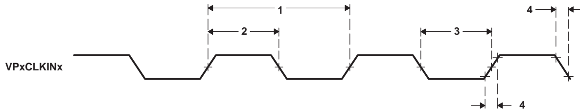
Figure 5–50. Video Port Display VPxCLKINx Timing
