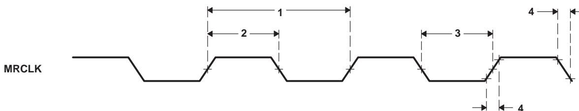
Figure 5–53. MRCLK Timing (EMAC – Receive)
