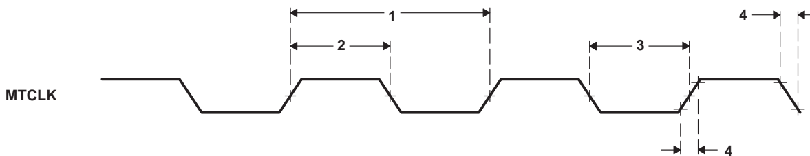
Figure 5–54. MTCLK Timing (EMAC – Transmit)
