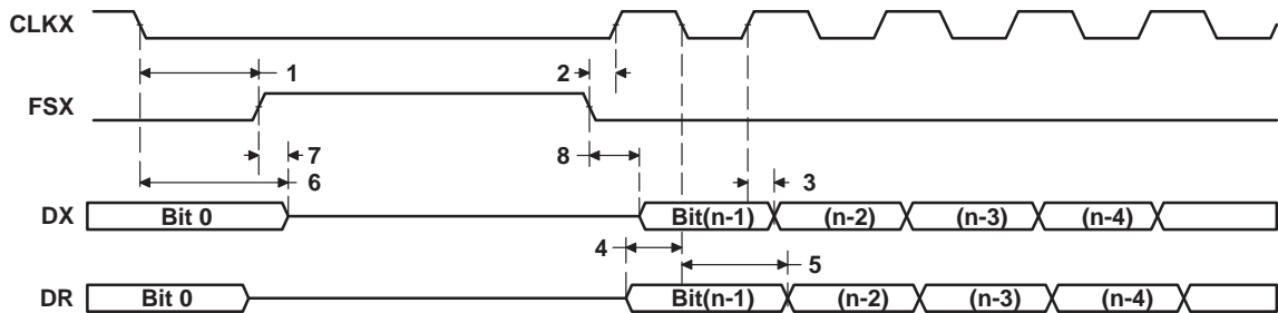
Figure 5–43. McBSP Timing as SPI Master or Slave: CLKSTP = 10b, CLKXP = 0
