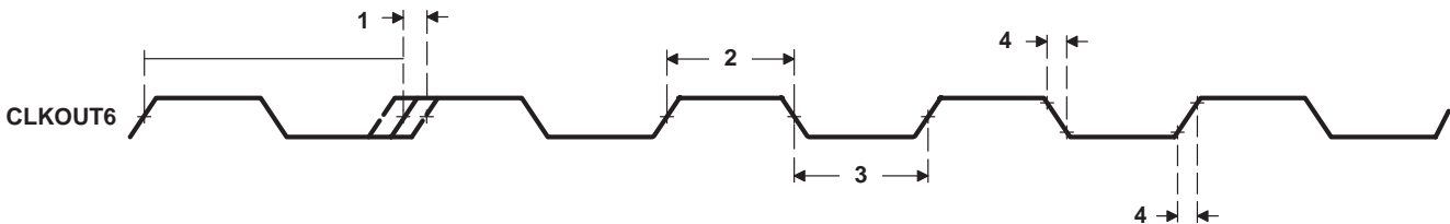
Figure 5–3. CLKOUT6 Timing
