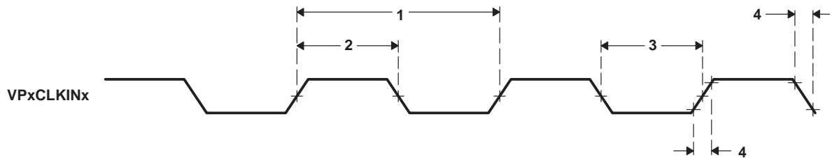
Figure 5–47. Video Port Capture VPxCLKINx Timing
