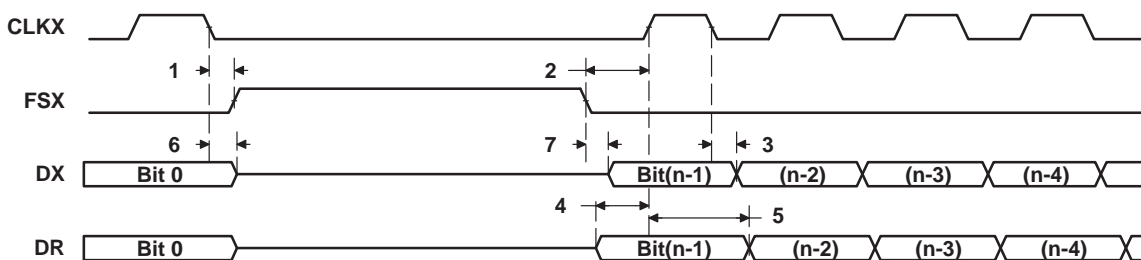
Figure 5–44. McBSP Timing as SPI Master or Slave: CLKSTP = 11b, CLKXP = 0
