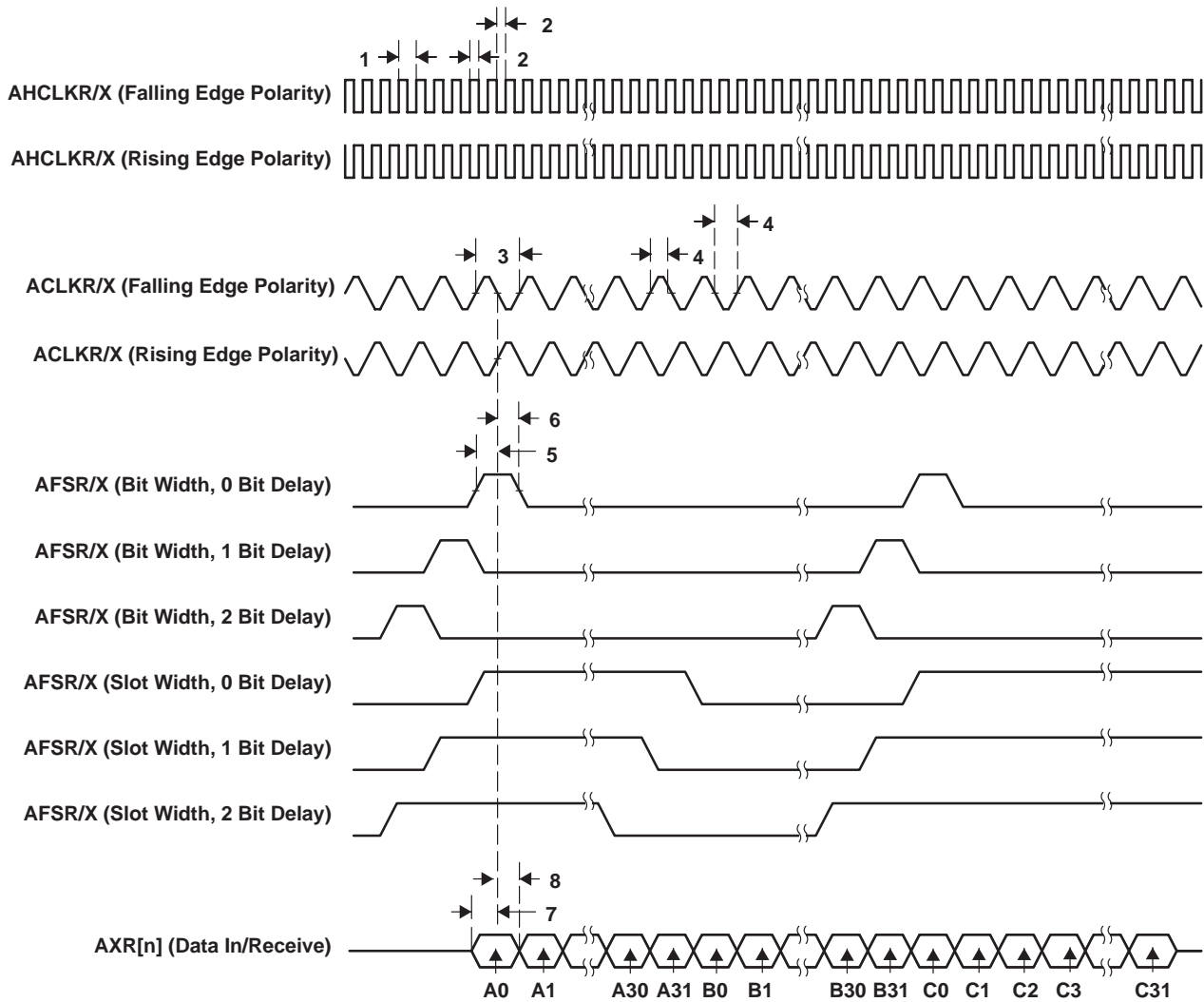
Figure 5-24. McASP Input Timings
