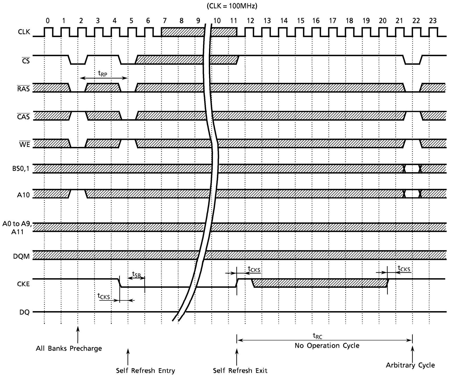
Figure 12. Self Refresh Cycle
