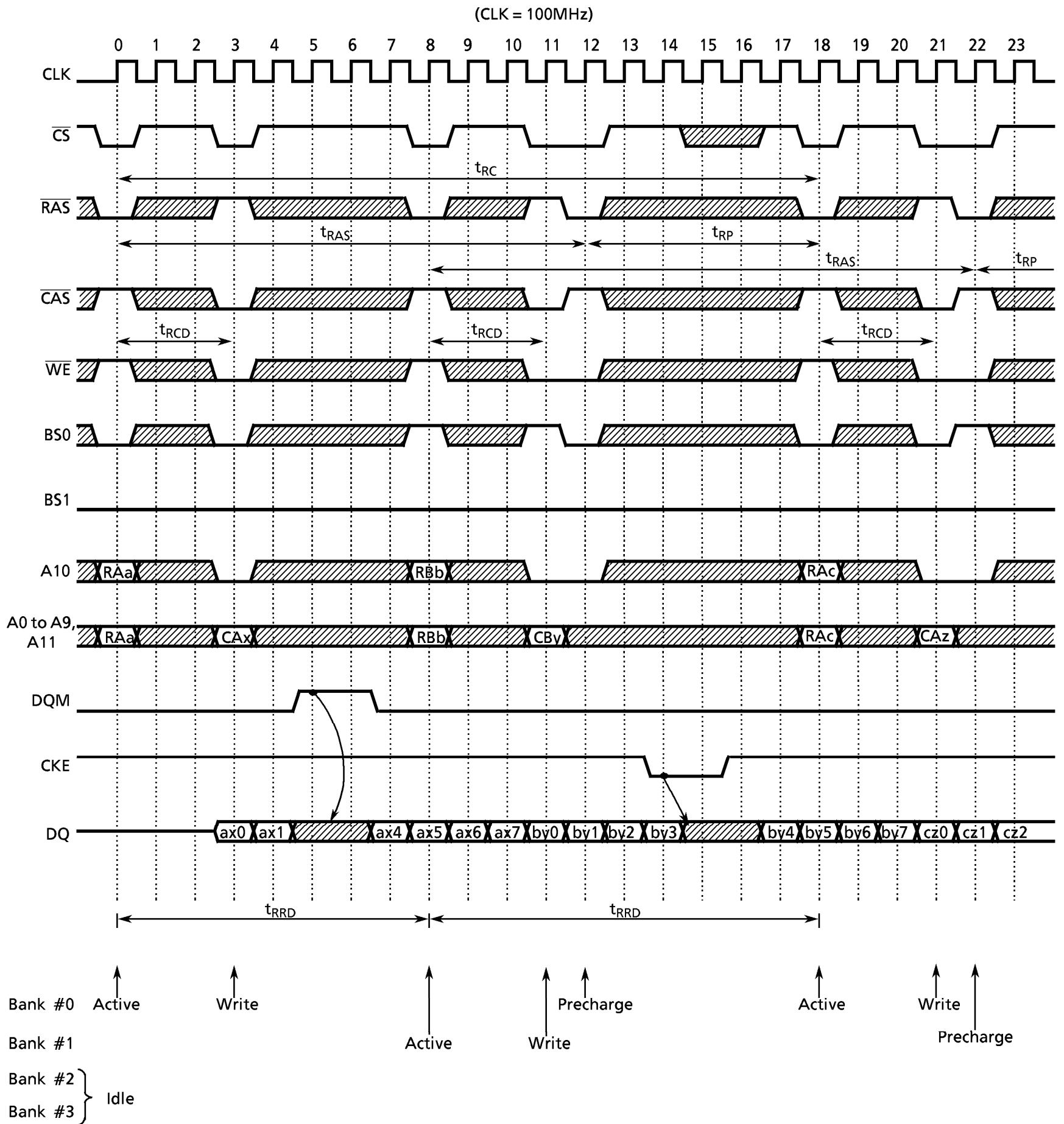
Figure 5. Interleaved Bank Write (Burst Length=8)
