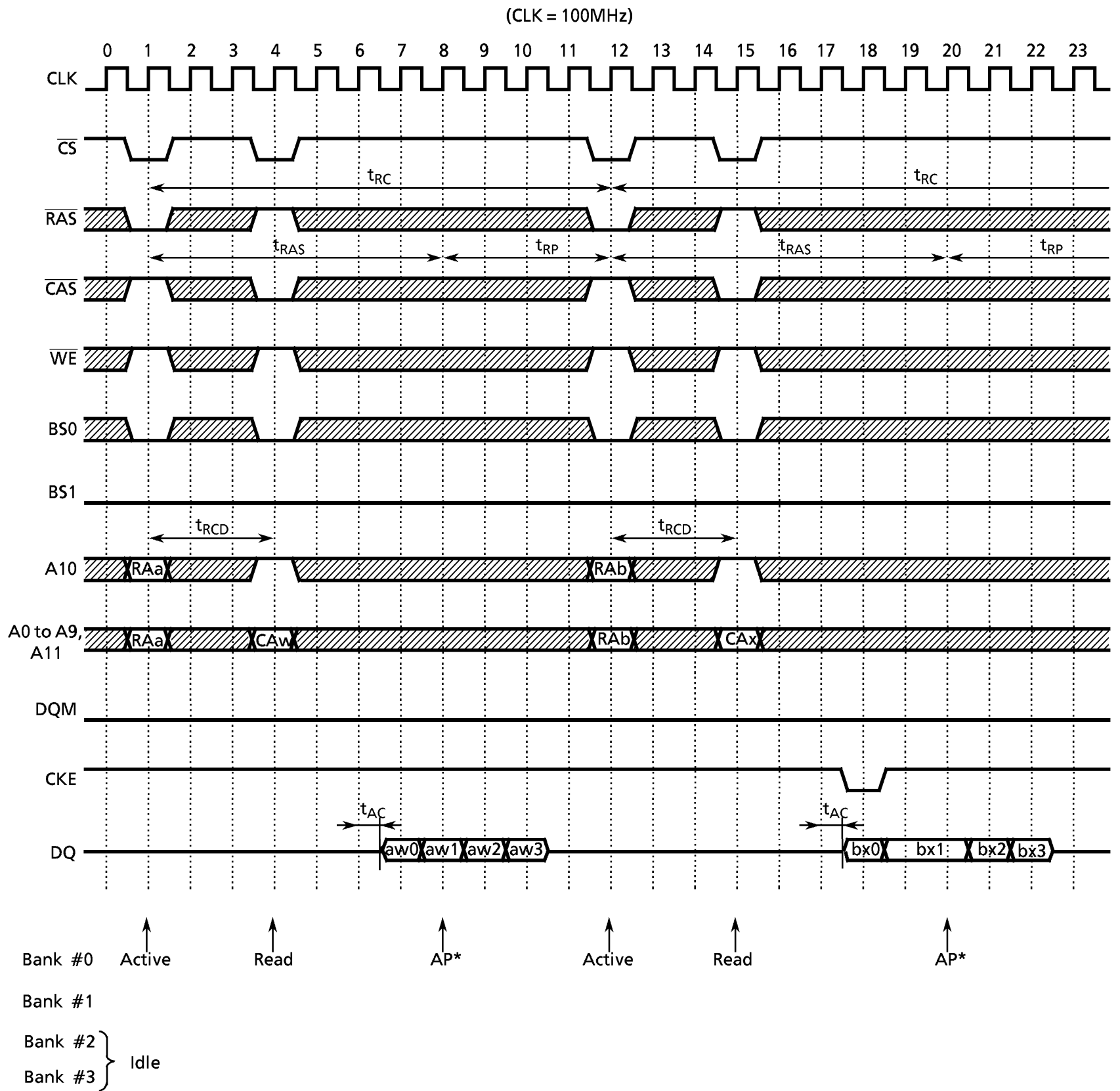
Figure 9. Auto Precharge Read (Burst Length=4, \overline{\text{CAS}} Latency=3)
