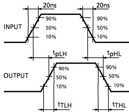
WAVEFORM
