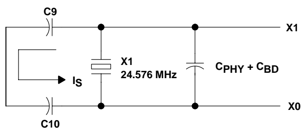
Figure 8–4. Load Capacitance for the TSB43AB22 PHY
