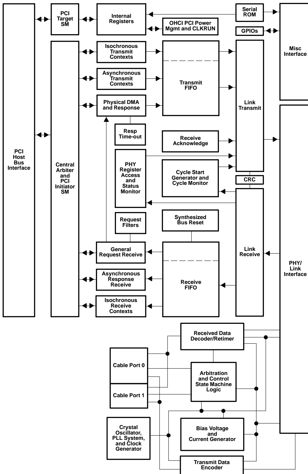
Figure 3–1. TSB43AB22 Block Diagram
