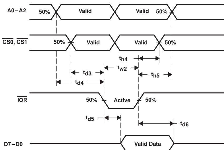
Figure 6. Read-Cycle Timing
