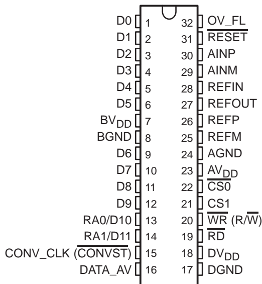
DA PACKAGE (TOP VIEW)
