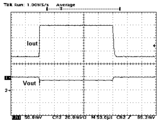
Figure 27 : Load Transient
