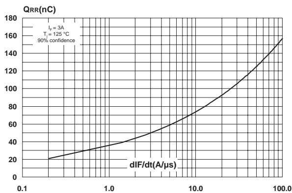
Fig. 6-2: Reverse recovery charges versus dI/dt (modulation diode).
