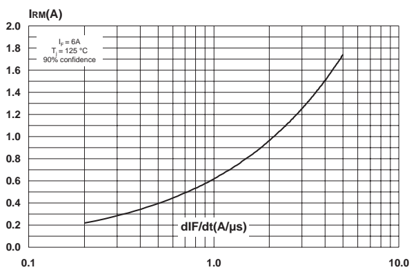
Fig. 7-1: Peak reverse recovery current versus dI/dt (damper diode).
