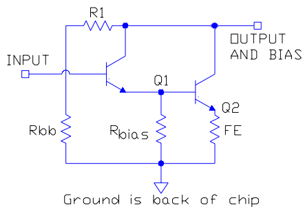
Simplified Schematic of MMIC
