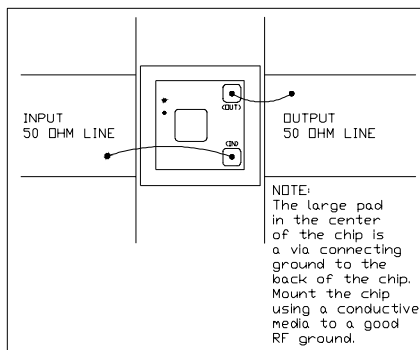
Suggested Bonding Arrangement
