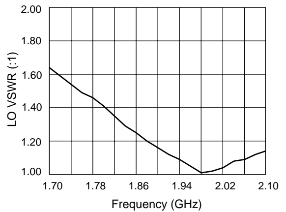
LO VSWR vs. Frequency
