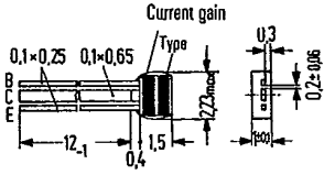
Approx. weight 20 mg Dimensions in mm
