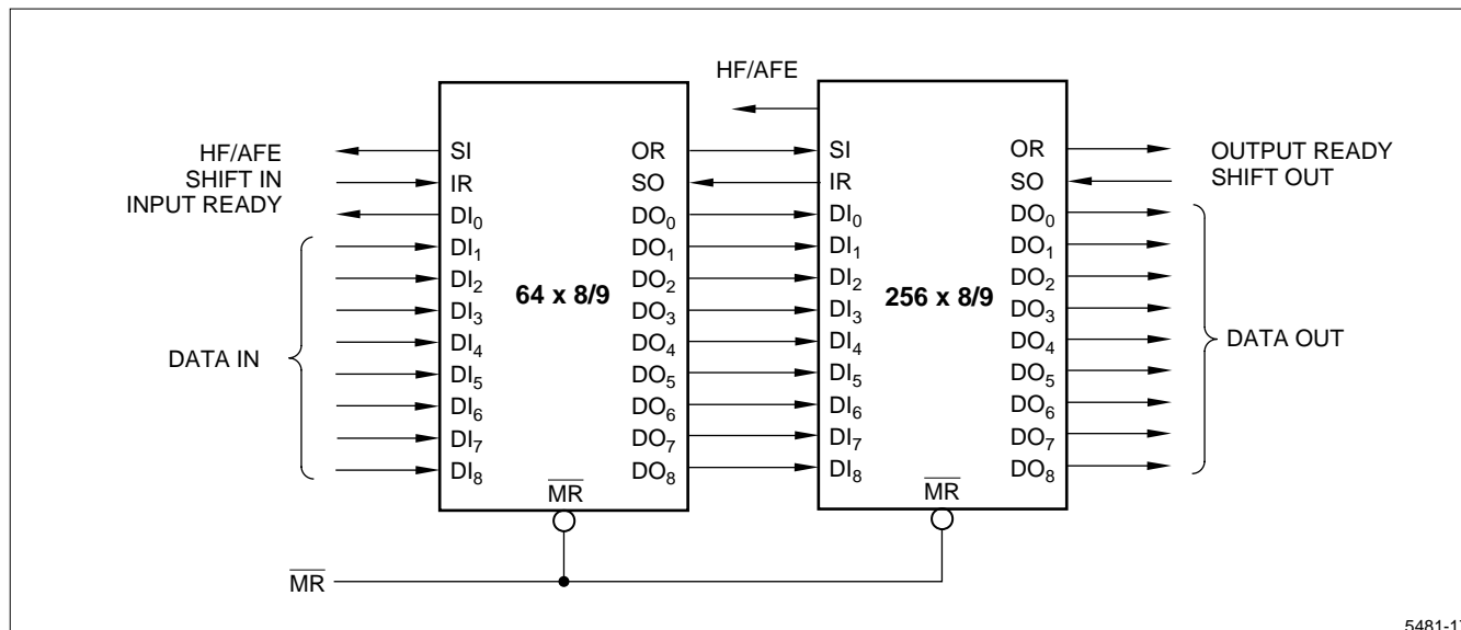
Figure 17. 128 × 8/9 Configuration
