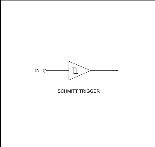
Figure 1-6. Pin Circuit Type B-4
