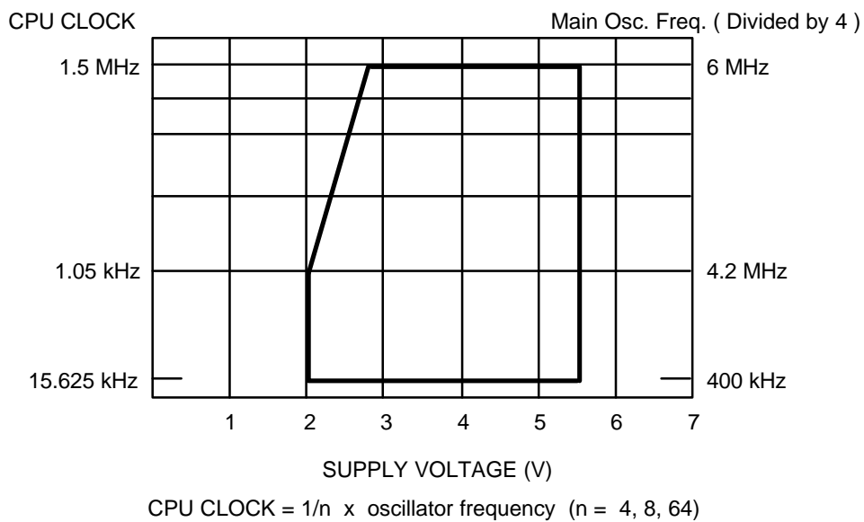
Figure 15-3. Standard Operating Voltage Range
