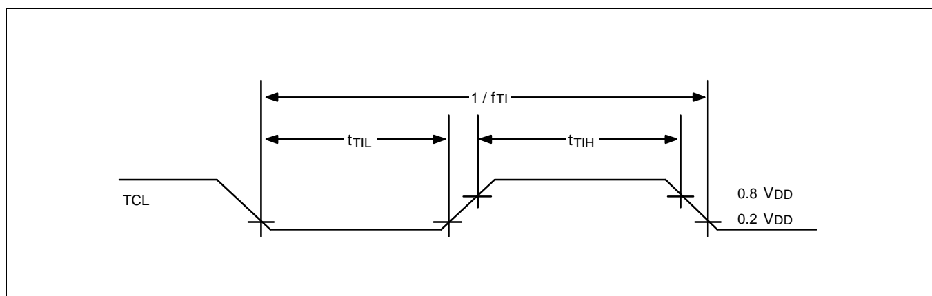
Figure 13-6. TCL Timing
