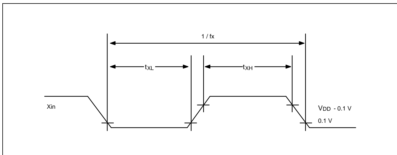
Figure 13-5. Clock Timing Measurement at X_{in}
