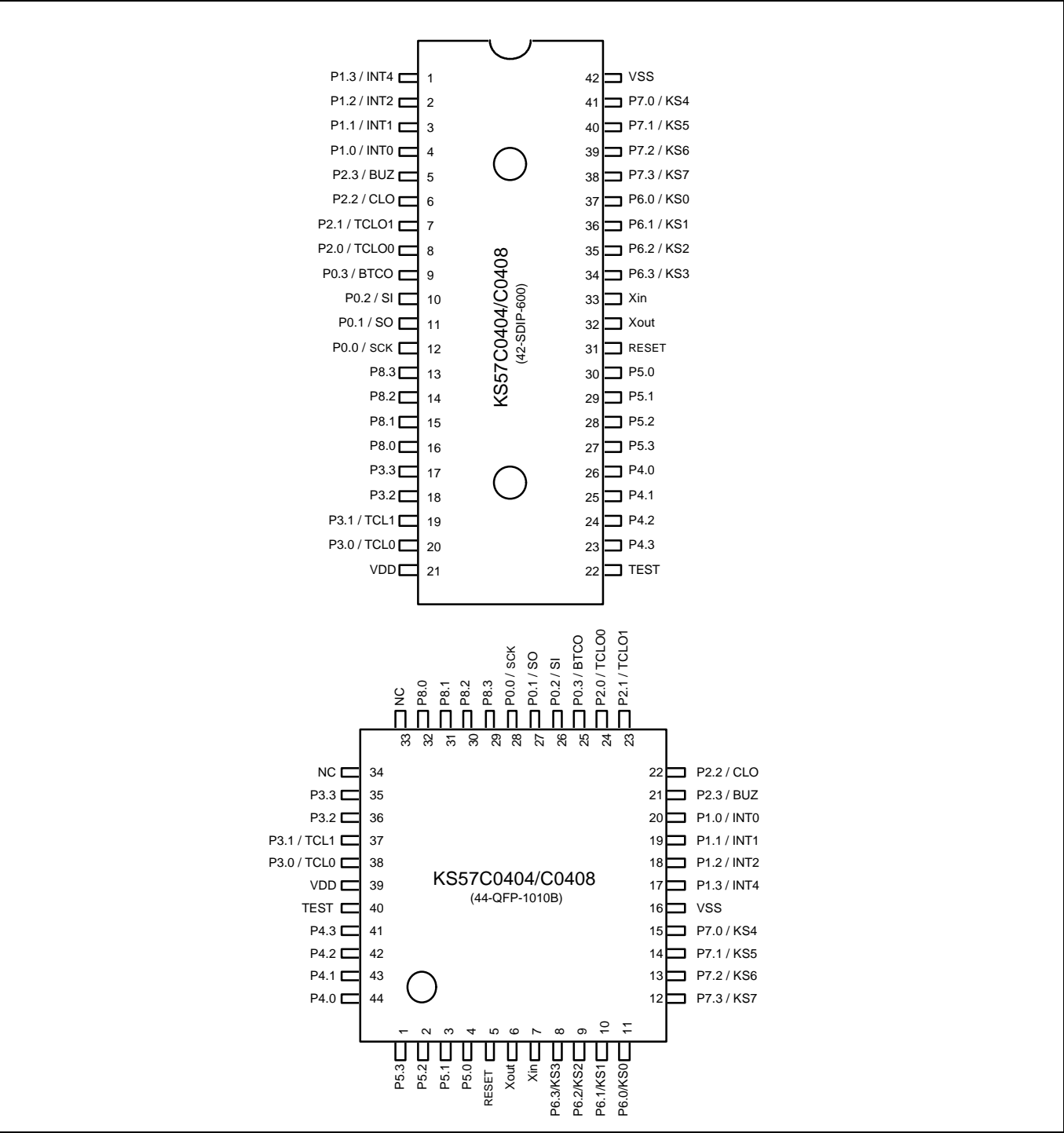
Figure 1–2. KS57C0404/C0408 Pin Assignment Diagrams
