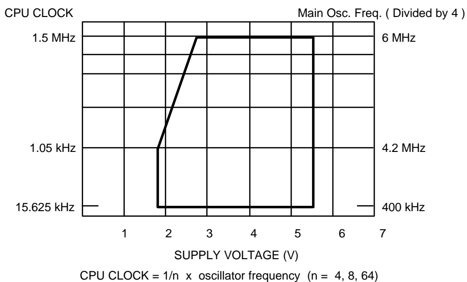
Figure 13-1. Standard Operating Voltage Range
