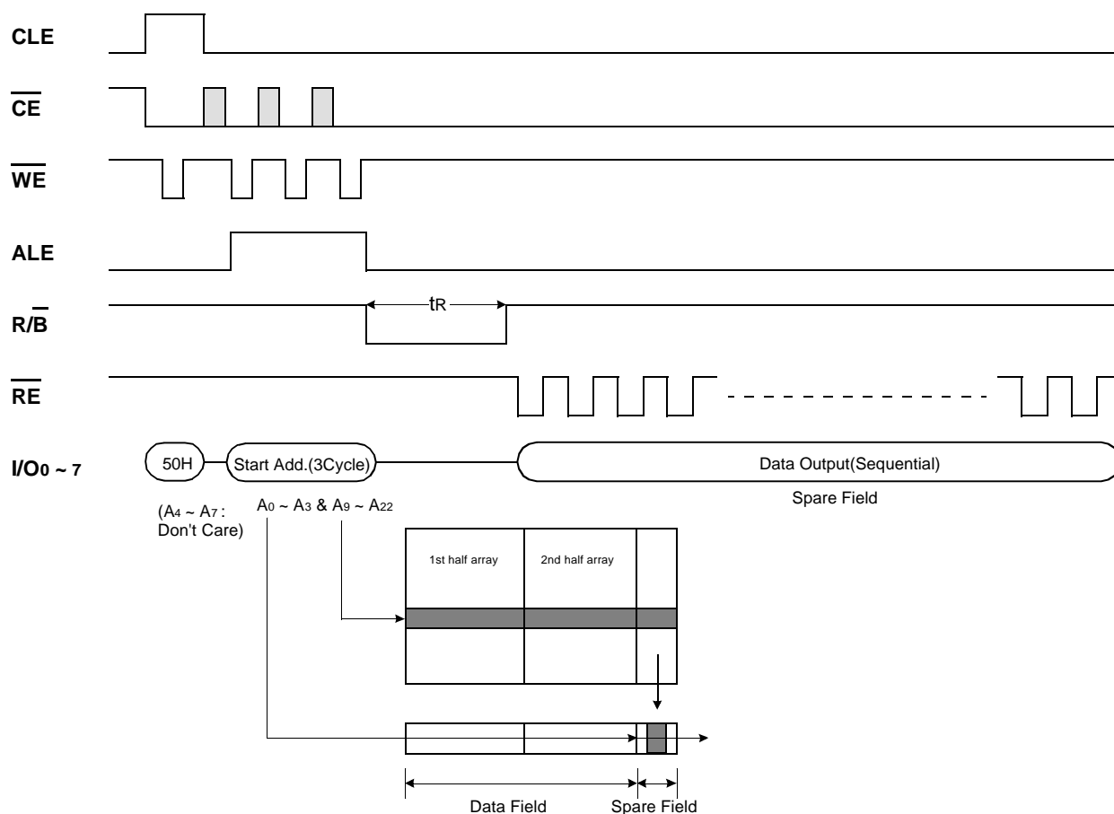
Figure 4. Read2 Operation
