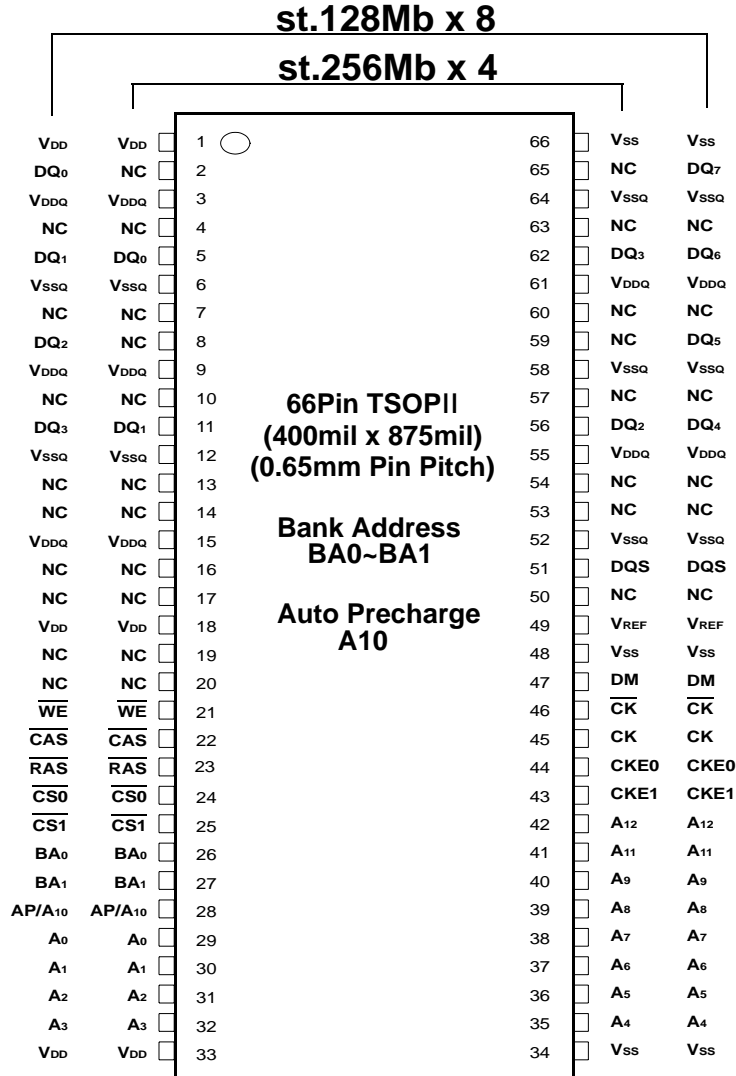
stacked 1Gb TSOP-II Package Pinout
