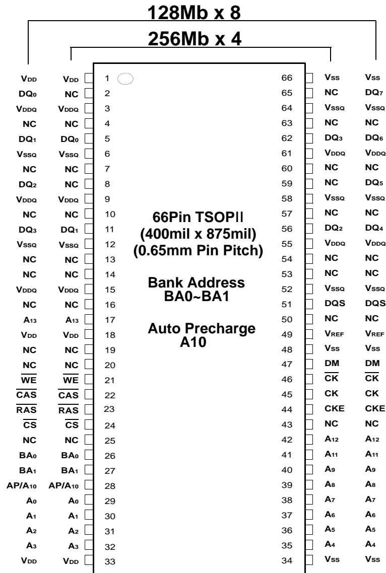
1Gb TSOP-II Package Pinout
