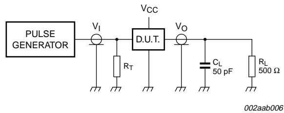
Fig 5. Load circuitry for switching times
