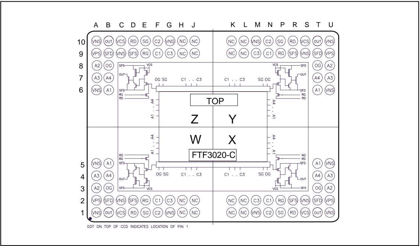
Figure 12 - FTF3020-C pin configuration (top view)
