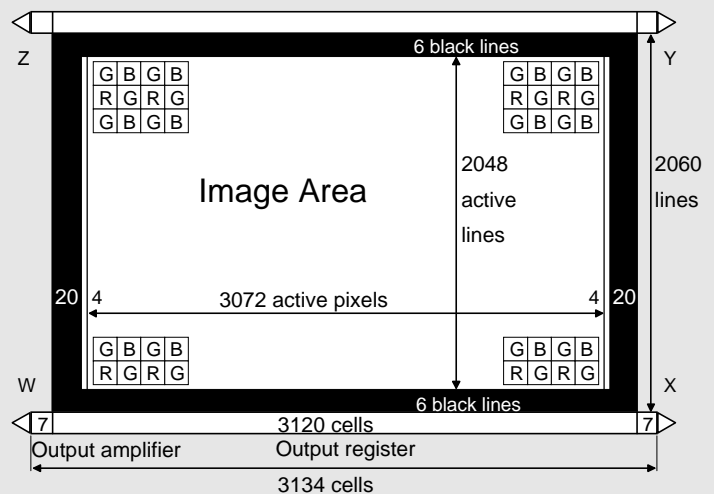
Figure 1 - Device structure
