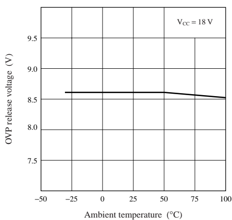
OVP release voltage characteristics
