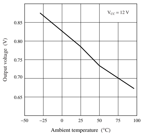
Pre-start low-level output voltage characteristics
