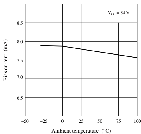
Operating bias current characteristics
