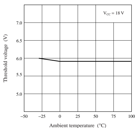
OVP operation threshold voltage characteristics
