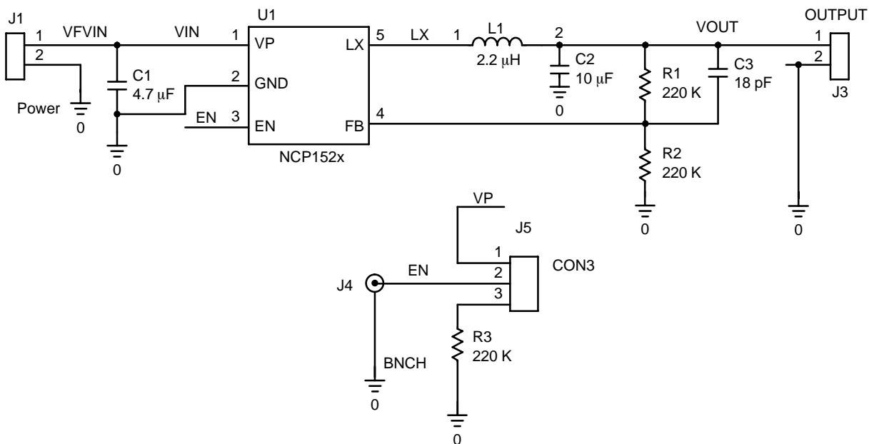
Figure 26. Schematics
