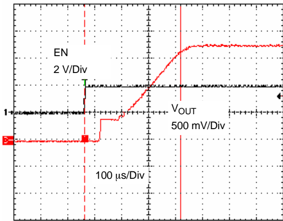
Figure 10. Soft Start Time ( V_{IN} = 3.6\text{ V} )
