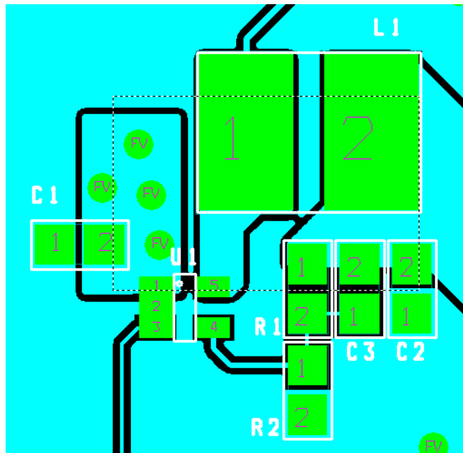
Figure 25. NCP1521 Board Layout
