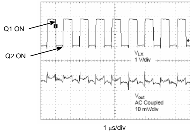
Figure 22. PWM Switching Waveform ( V_{in} = 3.6 \text{ V} , V_{out} = 1.8 \text{ V} , I_{out} = 300 \text{ mA} )
