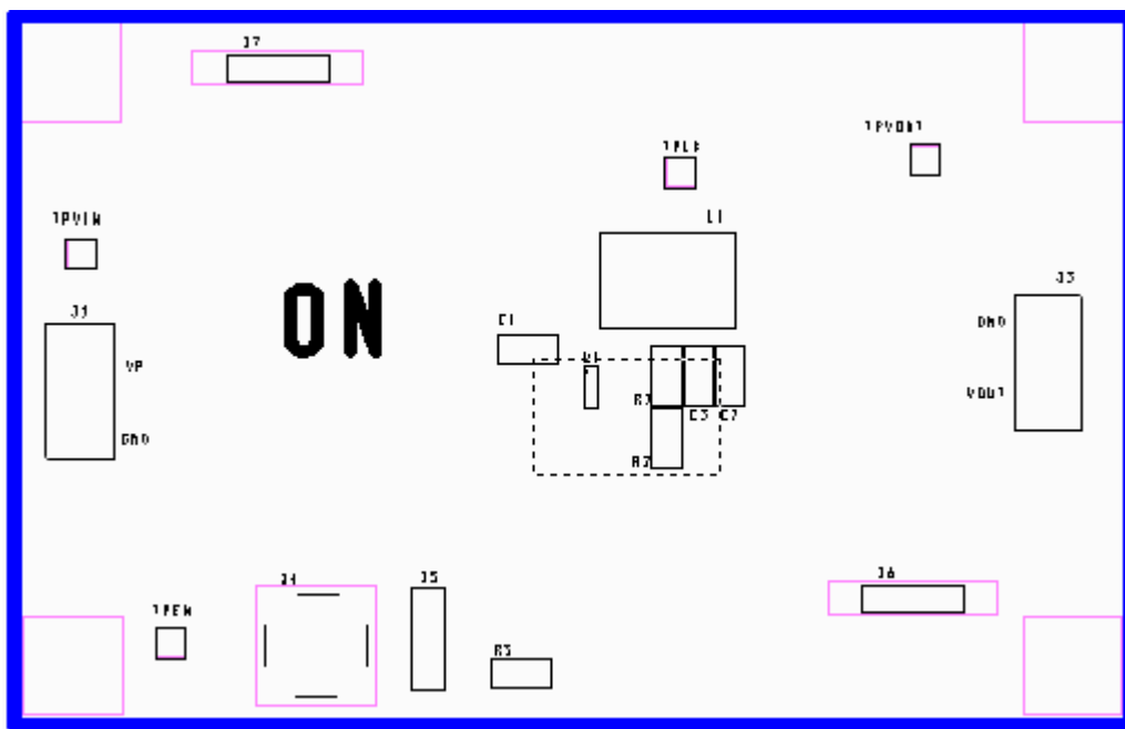
Figure 27. Silkscreen Layer
