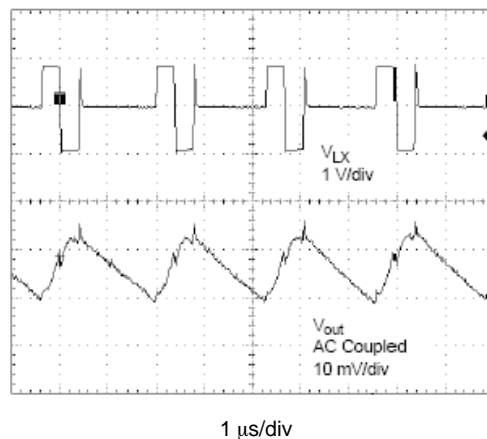
Figure 23. PFM Mode Switching Waveform ( V_{in} = 3.6 \text{ V} , V_{out} = 1.8 \text{ V} , I_{out} = 30 \text{ mA} )
