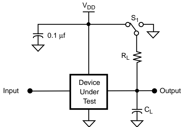
Figure 49. AC Test Conditions, T_A = 0^\circ\text{C} to 70^\circ\text{C} , V_{DD} = 5.0\text{V} \pm 10\%
