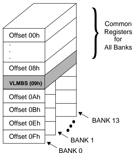
Figure 38. Register Bank Architecture
