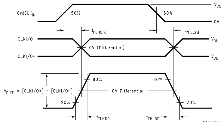
FIGURE 7. Driver Propagation Delay and Transition Time Waveforms
