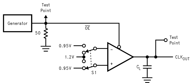
FIGURE 3. Output Enable ( \overline{OE} ) Delay Test Circuit
