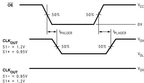
FIGURE 4. Output Enable ( \overline{OE} ) Delay Waveforms
