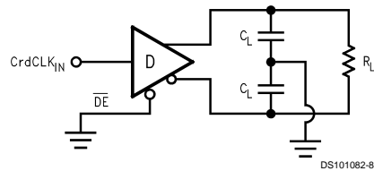
FIGURE 6. Driver Propagation Delay Test Circuit
