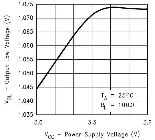
Output Low Voltage vs Power Supply Voltage
