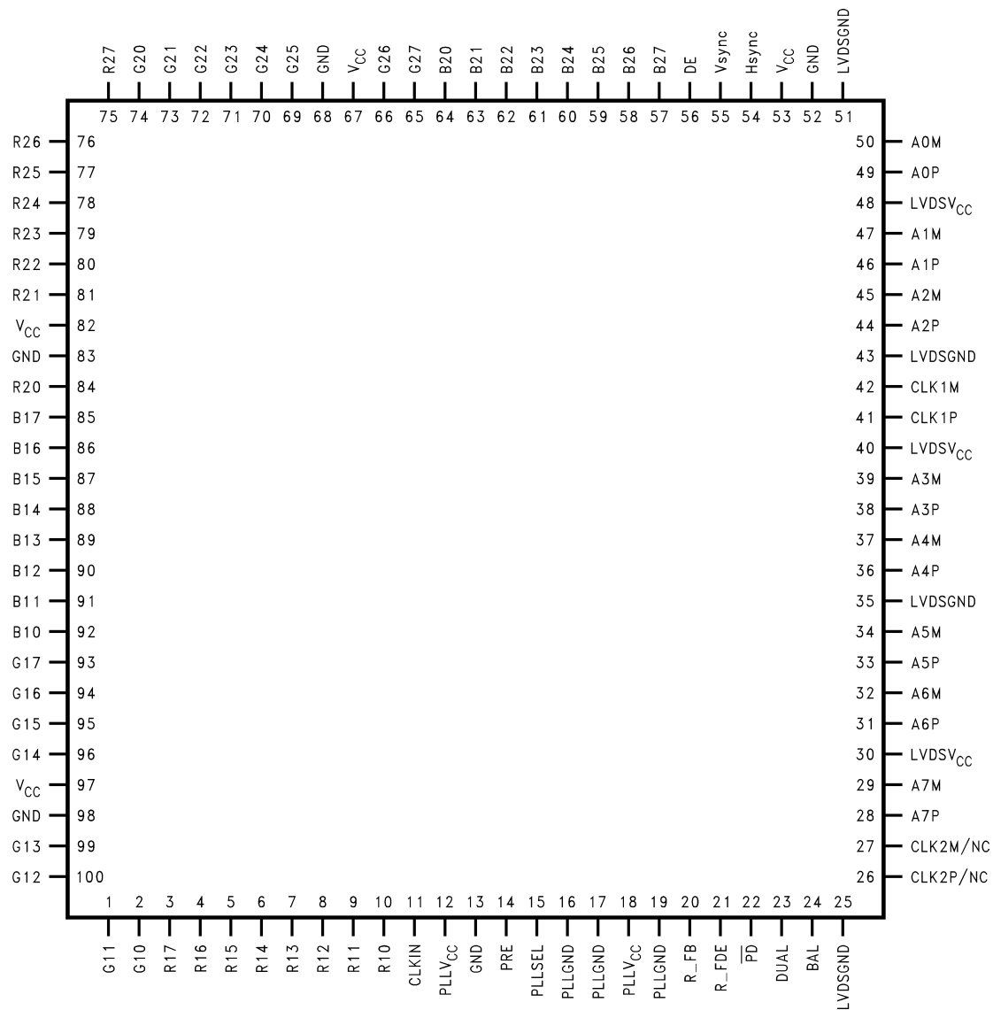
Transmitter-DS90C387
