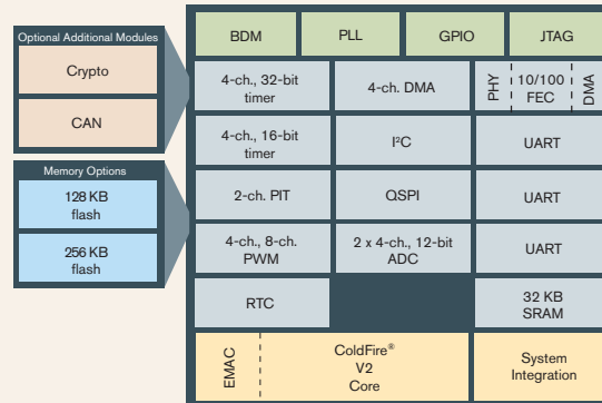
MCF5223X BLOCK DIAGRAM
