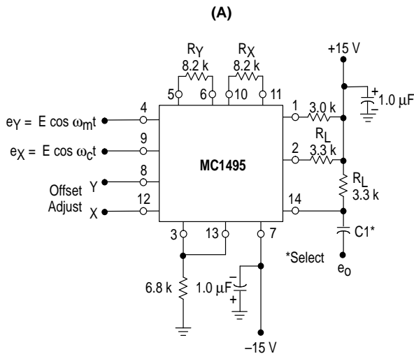
Figure 29. Balanced Modulator
