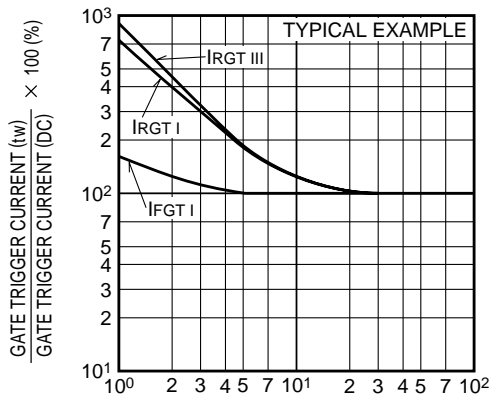
GATE TRIGGER CURRENT VS. GATE CURRENT PULSE WIDTH
