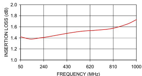
JTX-4-10T INSERTION LOSS
