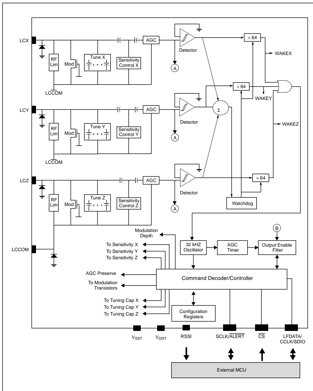
FIGURE 5-1: Functional Block Diagram.
