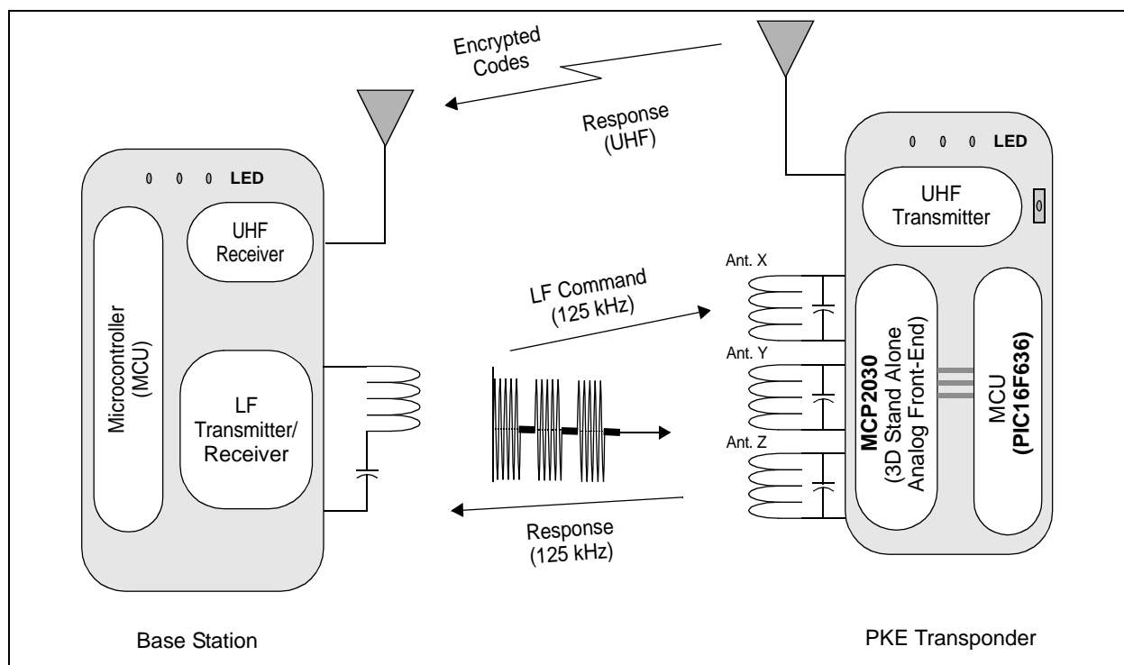
FIGURE 4-3: Example of Bidirectional Hand-free Passive Keyless Entry (PKE) System.
