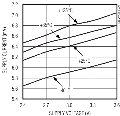
SUPPLY CURRENT vs. SUPPLY VOLTAGE (1x I_{LNA} )
