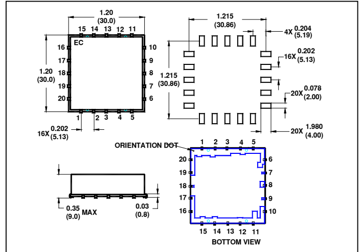
SM-85 Case Style
