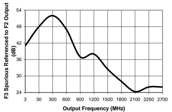
Spurious Response
