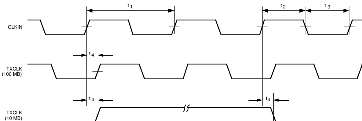
Figure 16. Output Timing
