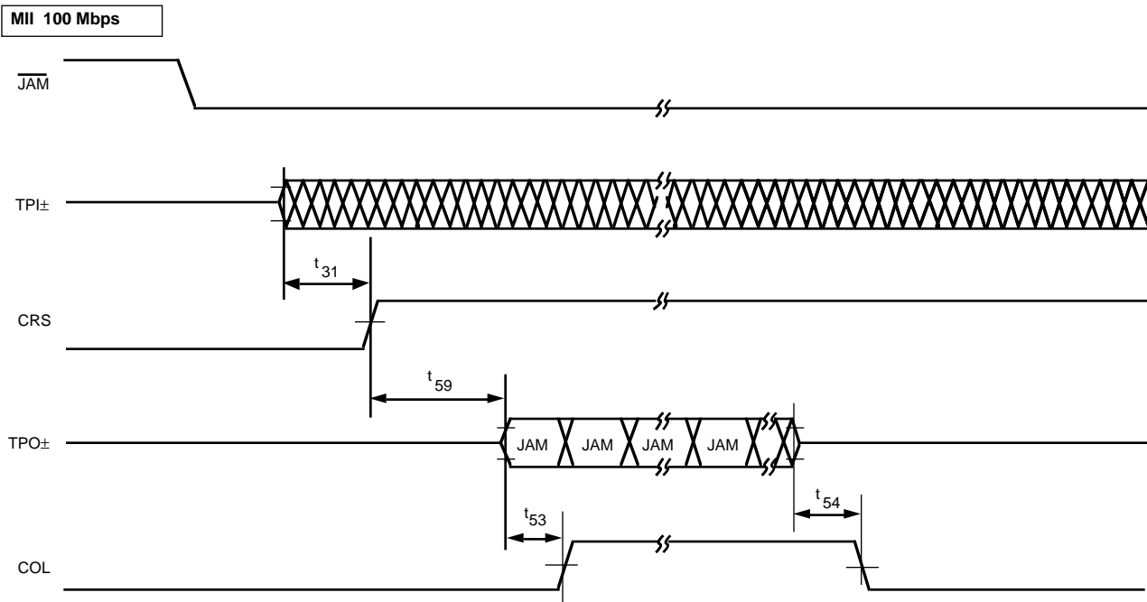
Figure 26. Jam Timing
