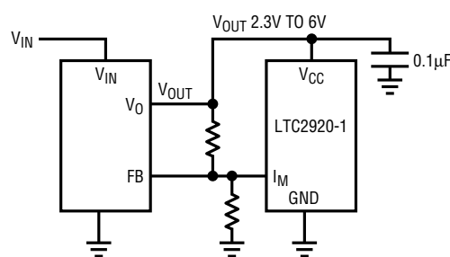
Figure 14. Connect LTC2920-1 to V_{OUT}
