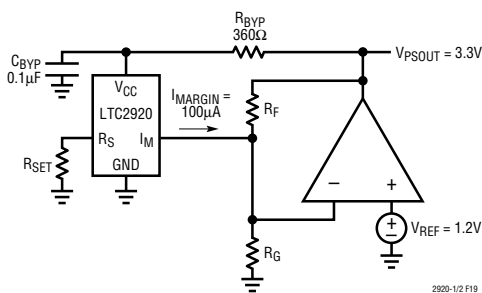
Figure 19. V_{CC} Power Filtering
