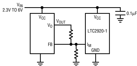
Figure 13. Connect LTC2920-1 to V_{IN}
